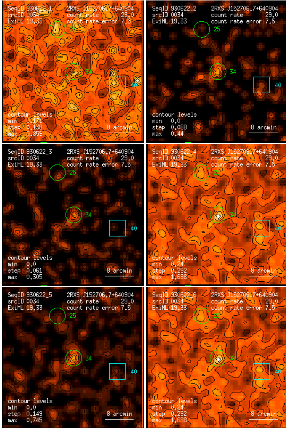
Figure 34: RASS 930622: detection 0034: band rate images, Gaussian filter: (1) PSPC channels 11 – 41, (2) 52 – 90, (3) 91 – 201, (4) 11 – 235, (5) 52 – 201, (6) 11 – 201. Broad band rates in counts/ks. Band rate contour levels in counts/ks/arcmin 2 .
