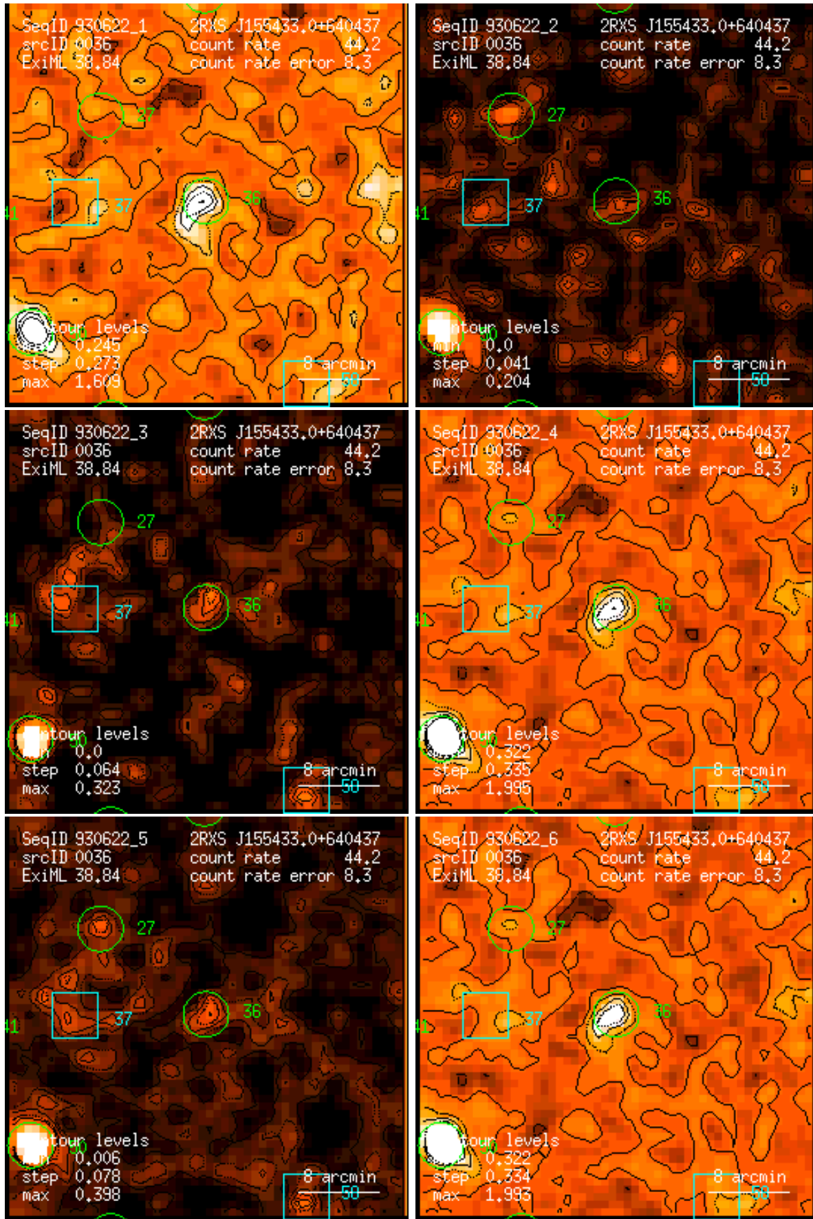
Figure 36: RASS 930622: detection 0036: band rate images, Gaussian filter: (1) PSPC channels 11 – 41, (2) 52 – 90, (3) 91 – 201, (4) 11 – 235, (5) 52 – 201, (6) 11 – 201. Broad band rates in counts/ks. Band rate contour levels in counts/ks/arcmin 2 .
