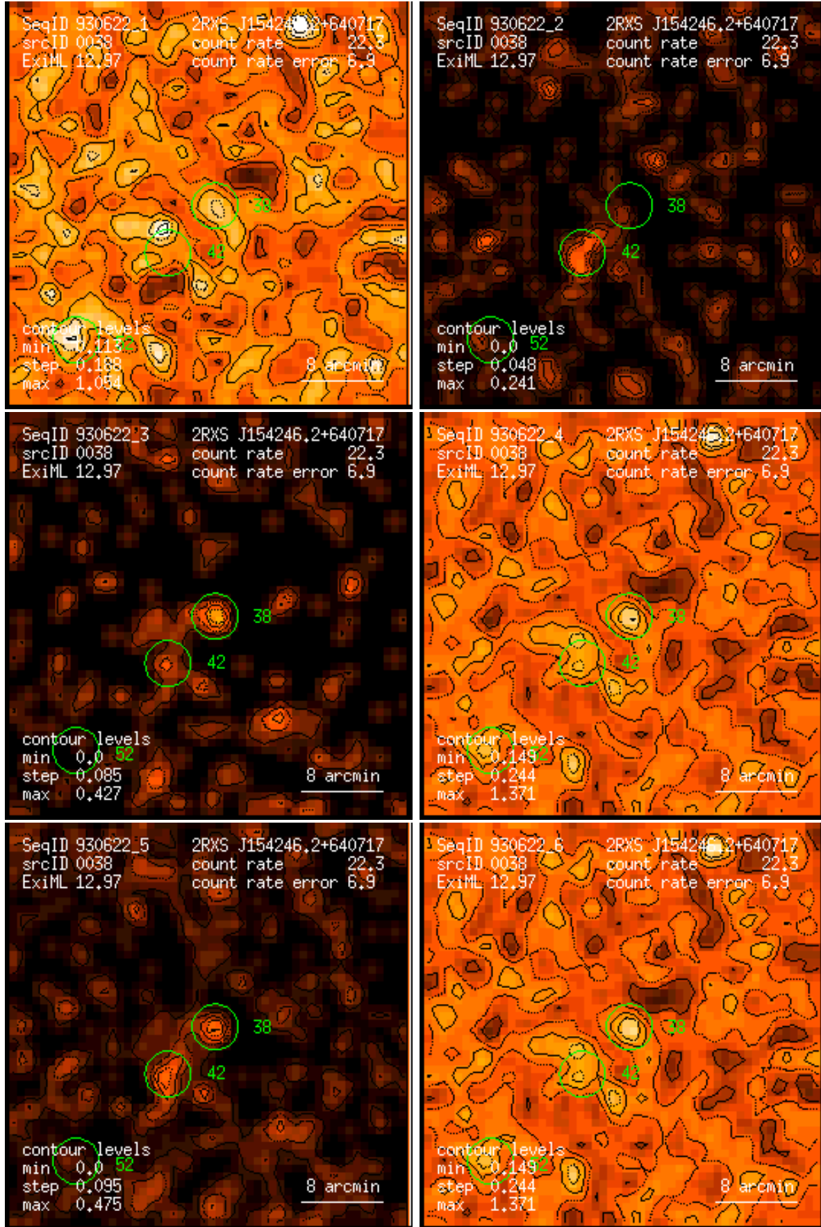
Figure 38: RASS 930622: detection 0038: band rate images, Gaussian filter: (1) PSPC channels 11 – 41, (2) 52 – 90, (3) 91 – 201, (4) 11 – 235, (5) 52 – 201, (6) 11 – 201. Broad band rates in counts/ks. Band rate contour levels in counts/ks/arcmin 2 .
