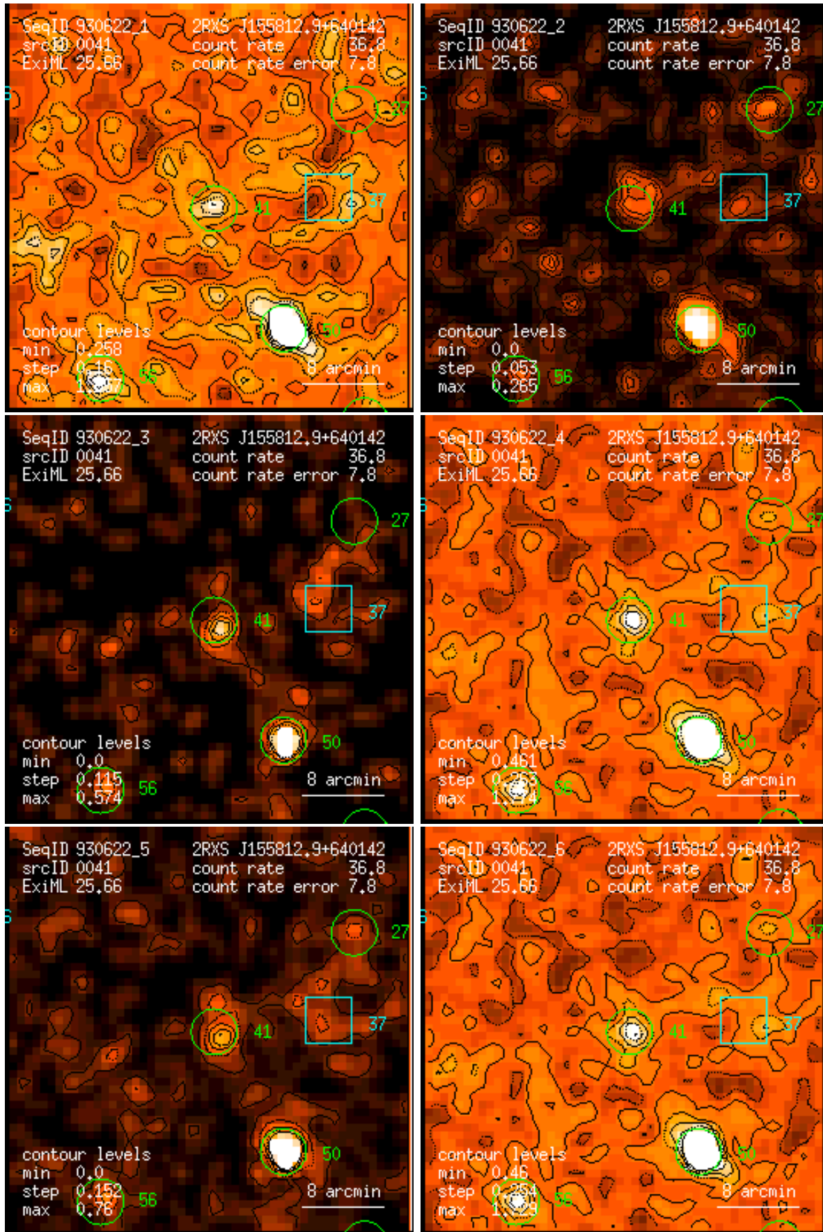
Figure 41: RASS 930622: detection 0041: band rate images, Gaussian filter: (1) PSPC channels 11 – 41, (2) 52 – 90, (3) 91 – 201, (4) 11 – 235, (5) 52 – 201, (6) 11 – 201. Broad band rates in counts/ks. Band rate contour levels in counts/ks/arcmin 2 .
