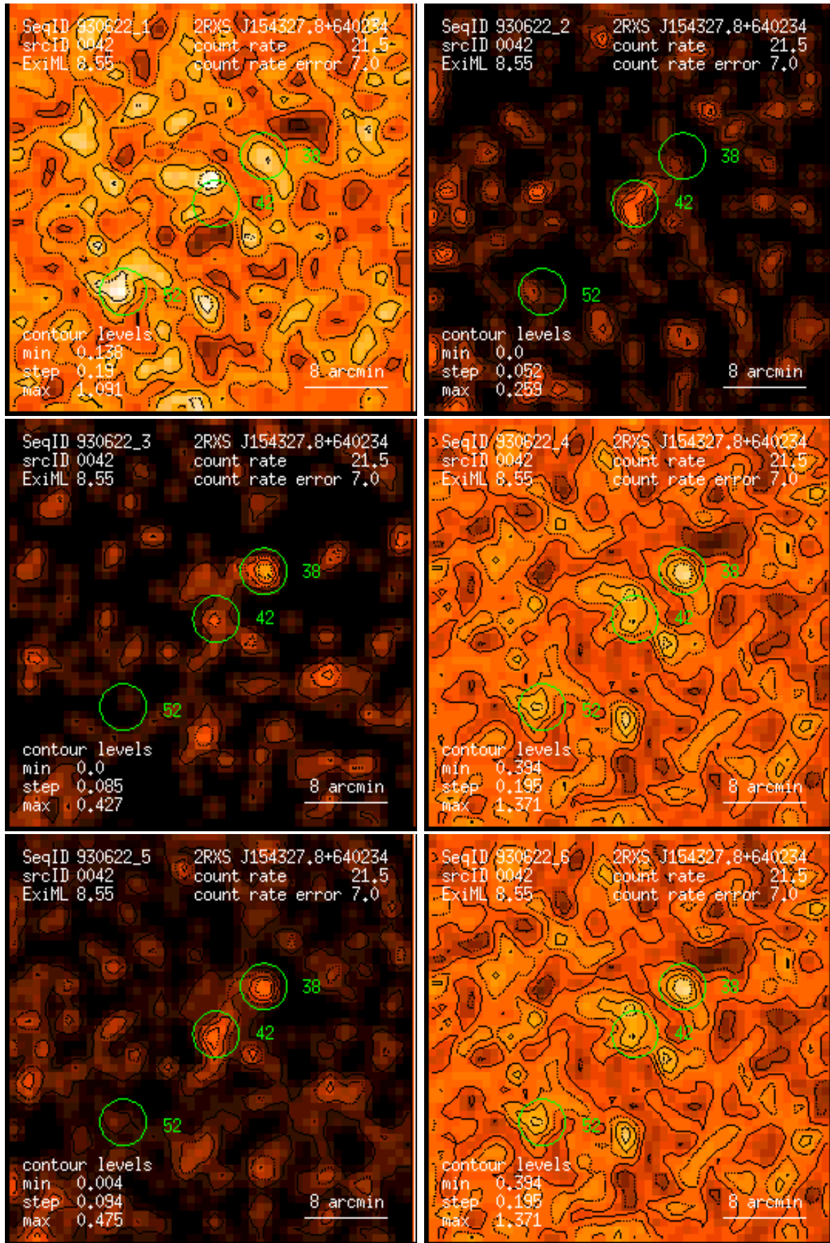
Figure 42: RASS 930622: detection 0042: band rate images, Gaussian filter: (1) PSPC channels 11 – 41, (2) 52 – 90, (3) 91 – 201, (4) 11 – 235, (5) 52 – 201, (6) 11 – 201. Broad band rates in counts/ks. Band rate contour levels in counts/ks/arcmin 2 .
