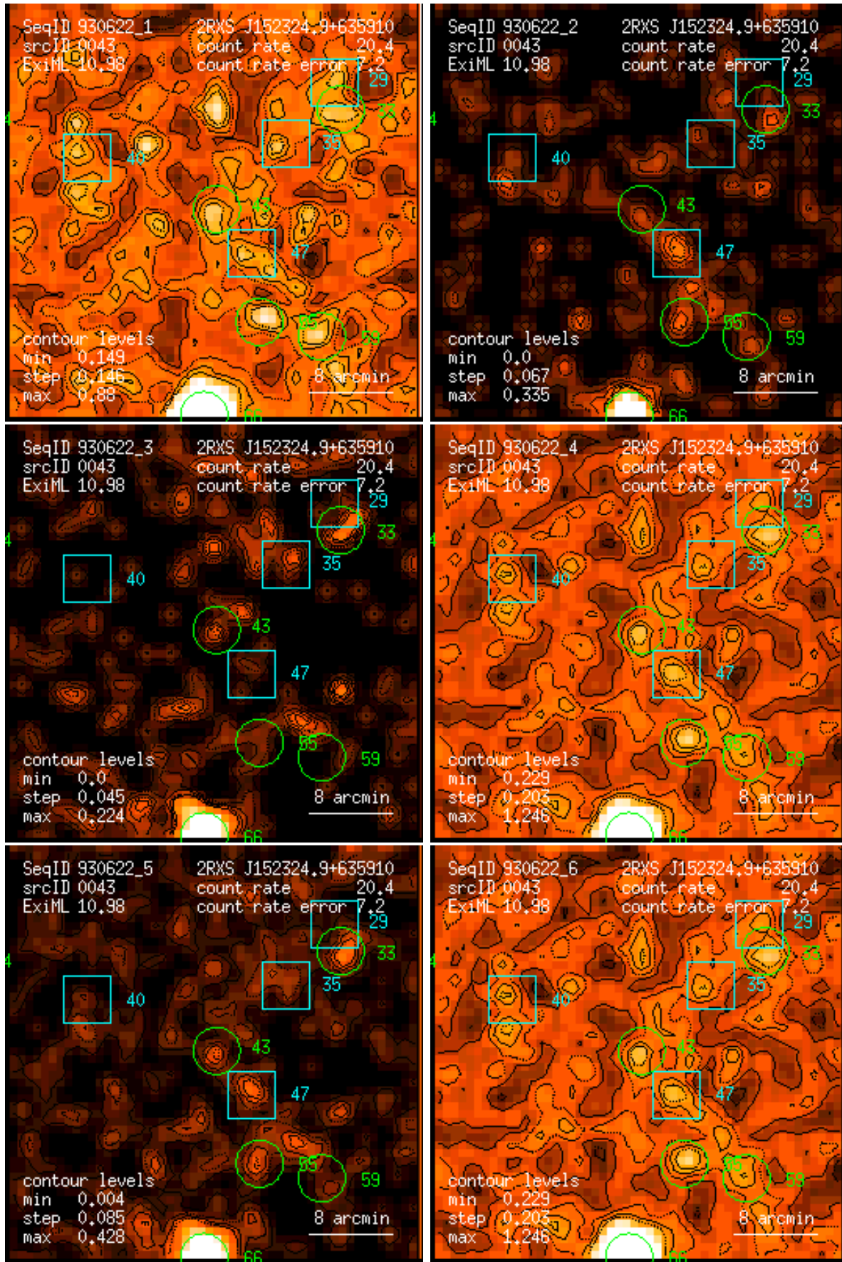
Figure 43: RASS 930622: detection 0043: band rate images, Gaussian filter: (1) PSPC channels 11 – 41, (2) 52 – 90, (3) 91 – 201, (4) 11 – 235, (5) 52 – 201, (6) 11 – 201. Broad band rates in counts/ks. Band rate contour levels in counts/ks/arcmin 2 .
