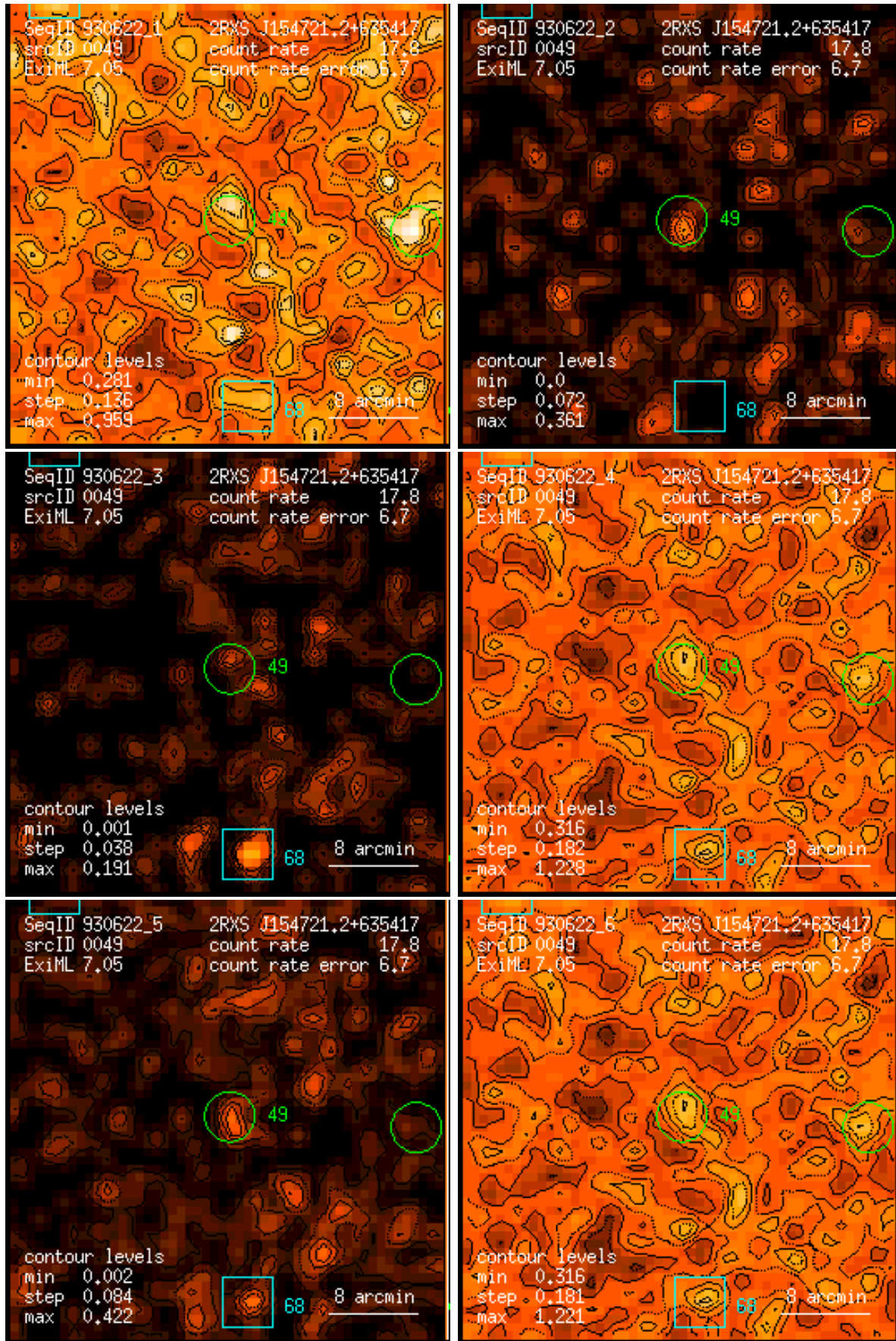
Figure 49: RASS 930622: detection 0049: band rate images, Gaussian filter: (1) PSPC channels 11 – 41, (2) 52 – 90, (3) 91 – 201, (4) 11 – 235, (5) 52 – 201, (6) 11 – 201. Broad band rates in counts/ks. Band rate contour levels in counts/ks/arcmin 2 .
