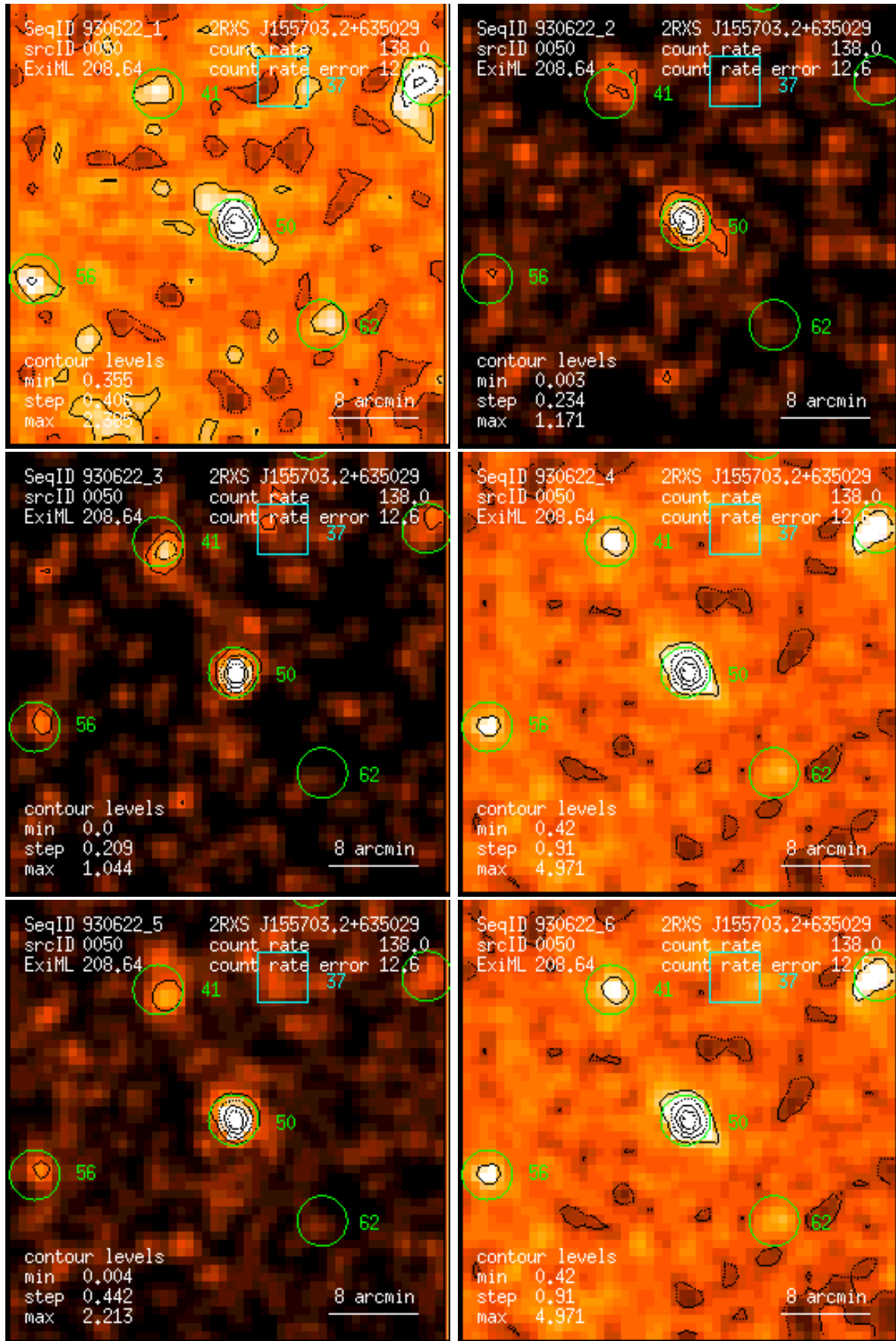
Figure 50: RASS 930622: detection 0050: band rate images, Gaussian filter: (1) PSPC channels 11 – 41, (2) 52 – 90, (3) 91 – 201, (4) 11 – 235, (5) 52 – 201, (6) 11 – 201. Broad band rates in counts/ks. Band rate contour levels in counts/ks/arcmin 2 .
