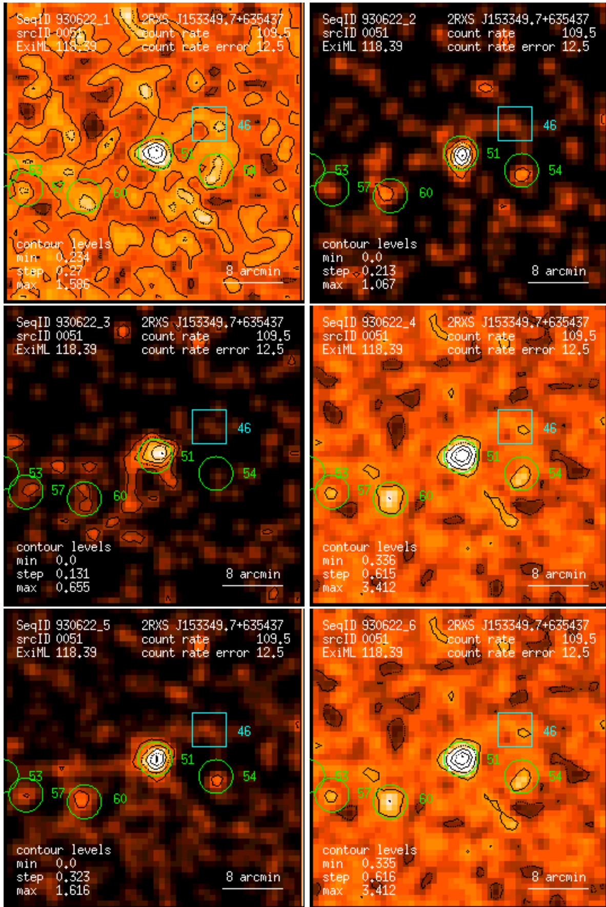
Figure 51: RASS 930622: detection 0051: band rate images, Gaussian filter: (1) PSPC channels 11 – 41, (2) 52 – 90, (3) 91 – 201, (4) 11 – 235, (5) 52 – 201, (6) 11 – 201. Broad band rates in counts/ks. Band rate contour levels in counts/ks/arcmin 2 .
