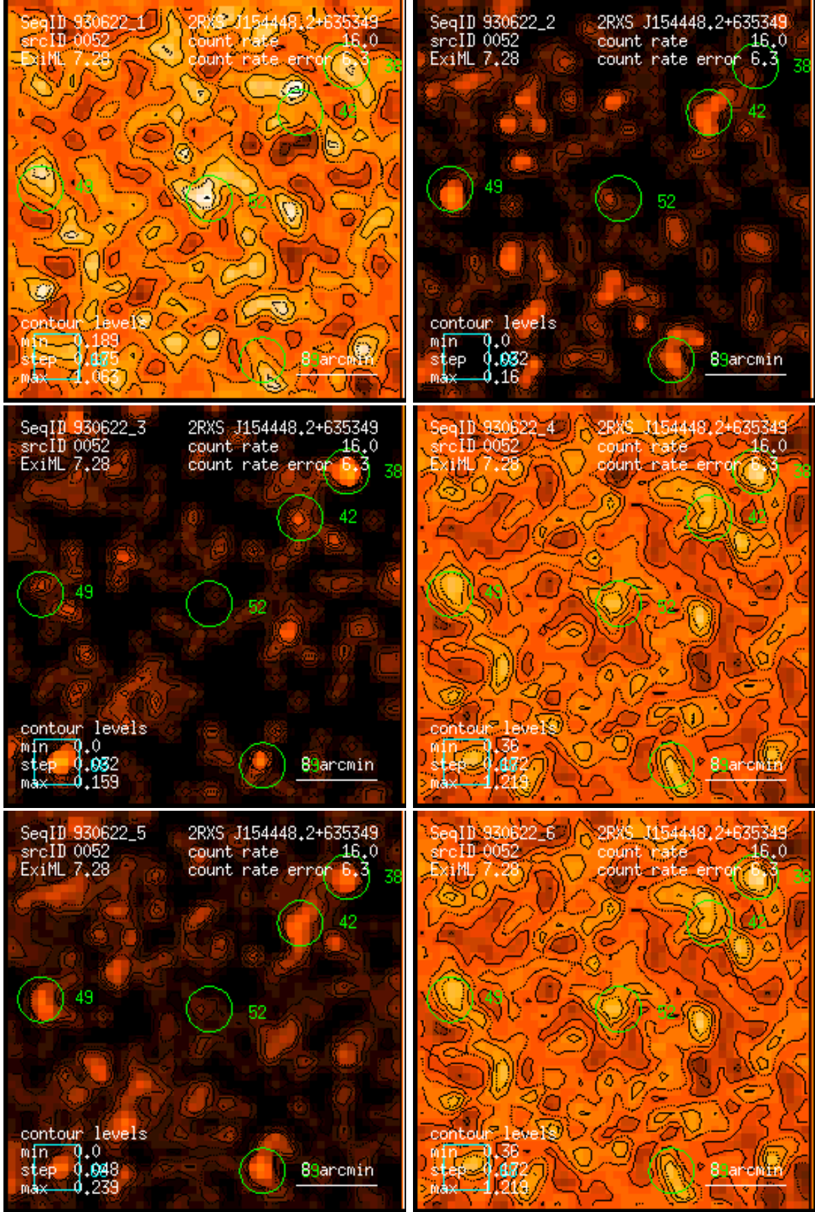
Figure 52: RASS 930622: detection 0052: band rate images, Gaussian filter: (1) PSPC channels 11 – 41, (2) 52 – 90, (3) 91 – 201, (4) 11 – 235, (5) 52 – 201, (6) 11 – 201. Broad band rates in counts/ks. Band rate contour levels in counts/ks/arcmin 2 .
