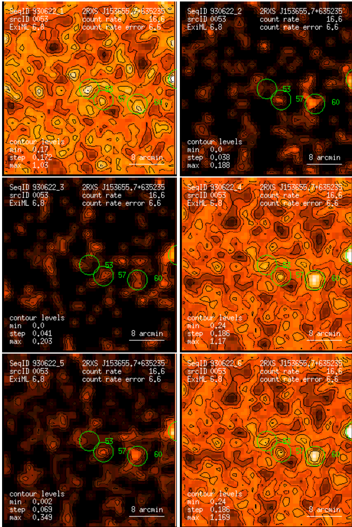
Figure 53: RASS 930622: detection 0053: band rate images, Gaussian filter: (1) PSPC channels 11 – 41, (2) 52 – 90, (3) 91 – 201, (4) 11 – 235, (5) 52 – 201, (6) 11 – 201. Broad band rates in counts/ks. Band rate contour levels in counts/ks/arcmin 2 .
