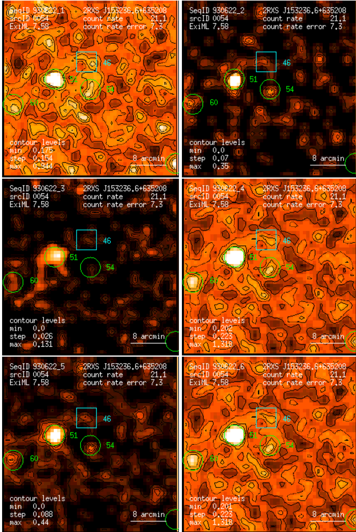
Figure 54: RASS 930622: detection 0054: band rate images, Gaussian filter: (1) PSPC channels 11 – 41, (2) 52 – 90, (3) 91 – 201, (4) 11 – 235, (5) 52 – 201, (6) 11 – 201. Broad band rates in counts/ks. Band rate contour levels in counts/ks/arcmin 2 .
