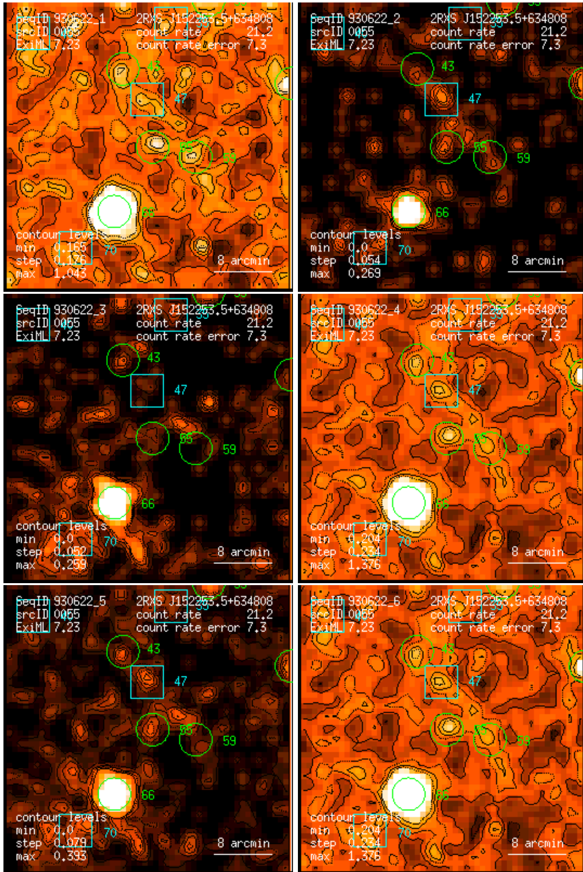
Figure 55: RASS 930622: detection 0055: band rate images, Gaussian filter: (1) PSPC channels 11 – 41, (2) 52 – 90, (3) 91 – 201, (4) 11 – 235, (5) 52 – 201, (6) 11 – 201. Broad band rates in counts/ks. Band rate contour levels in counts/ks/arcmin 2 .
