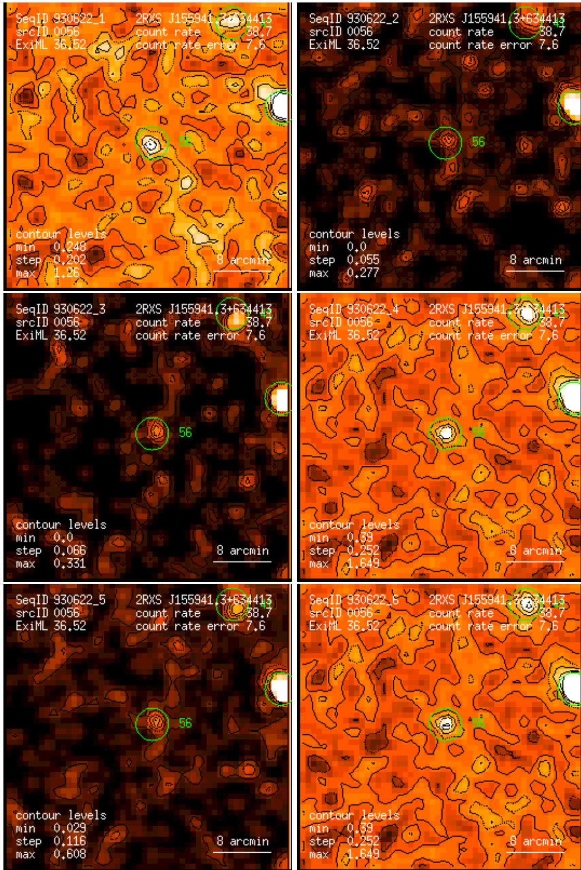
Figure 56: RASS 930622: detection 0056: band rate images, Gaussian filter: (1) PSPC channels 11 – 41, (2) 52 – 90, (3) 91 – 201, (4) 11 – 235, (5) 52 – 201, (6) 11 – 201. Broad band rates in counts/ks. Band rate contour levels in counts/ks/arcmin 2 .
