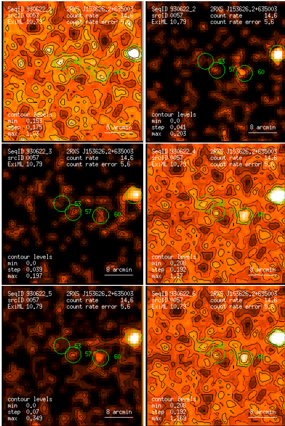
Figure 57: RASS 930622: detection 0057: band rate images, Gaussian filter: (1) PSPC channels 11 – 41, (2) 52 – 90, (3) 91 – 201, (4) 11 – 235, (5) 52 – 201, (6) 11 – 201. Broad band rates in counts/ks. Band rate contour levels in counts/ks/arcmin 2 .
