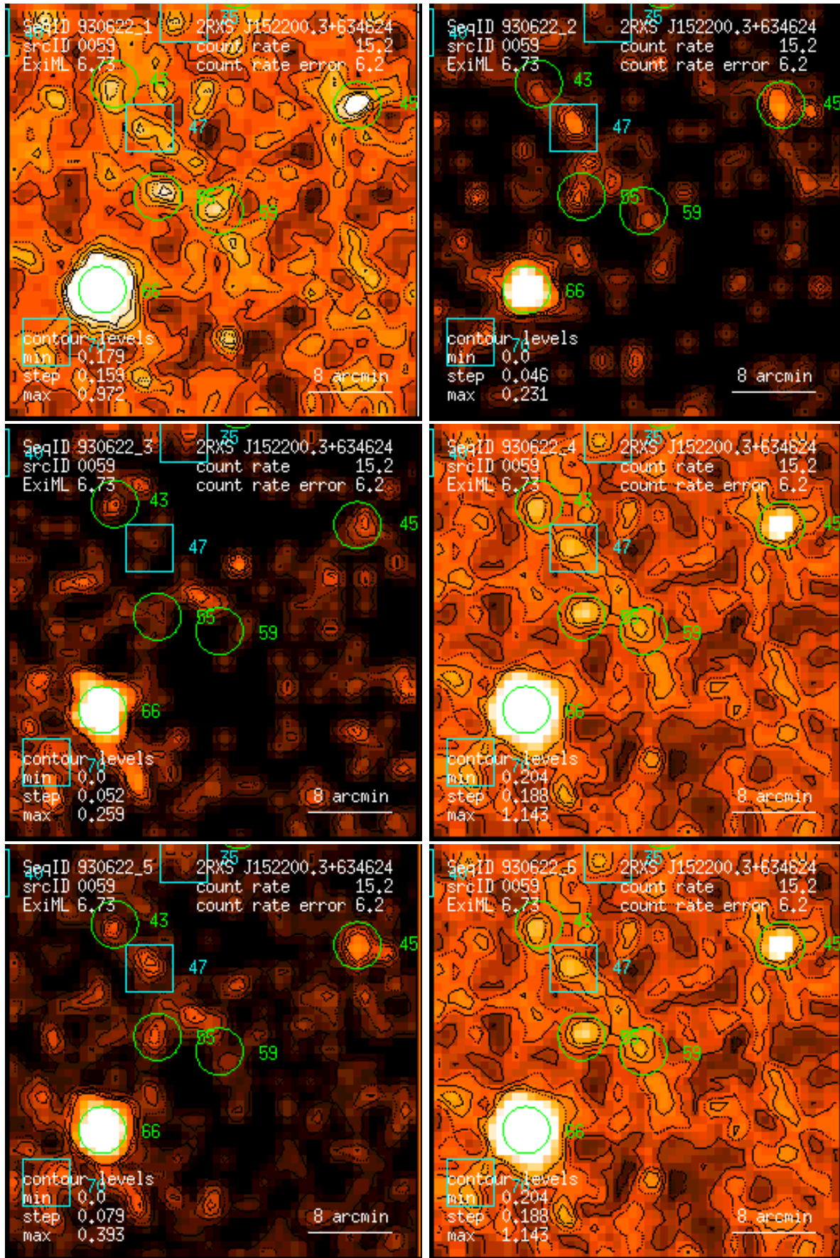
Figure 59: RASS 930622: detection 0059: band rate images, Gaussian filter: (1) PSPC channels 11 – 41, (2) 52 – 90, (3) 91 – 201, (4) 11 – 235, (5) 52 – 201, (6) 11 – 201. Broad band rates in counts/ks. Band rate contour levels in counts/ks/arcmin 2 .
