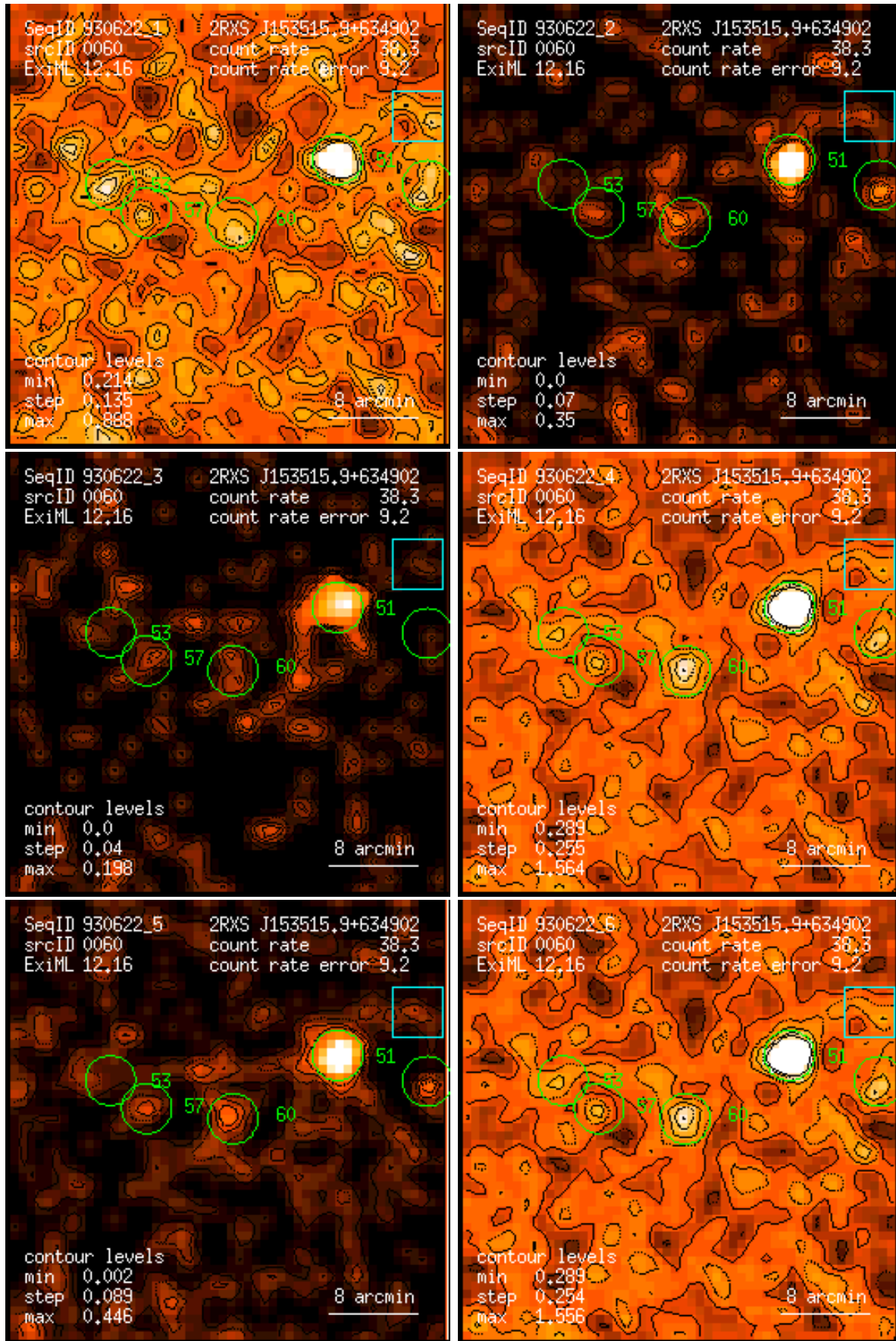
Figure 60: RASS 930622: detection 0060: band rate images, Gaussian filter: (1) PSPC channels 11 – 41, (2) 52 – 90, (3) 91 – 201, (4) 11 – 235, (5) 52 – 201, (6) 11 – 201. Broad band rates in counts/ks. Band rate contour levels in counts/ks/arcmin 2 .
