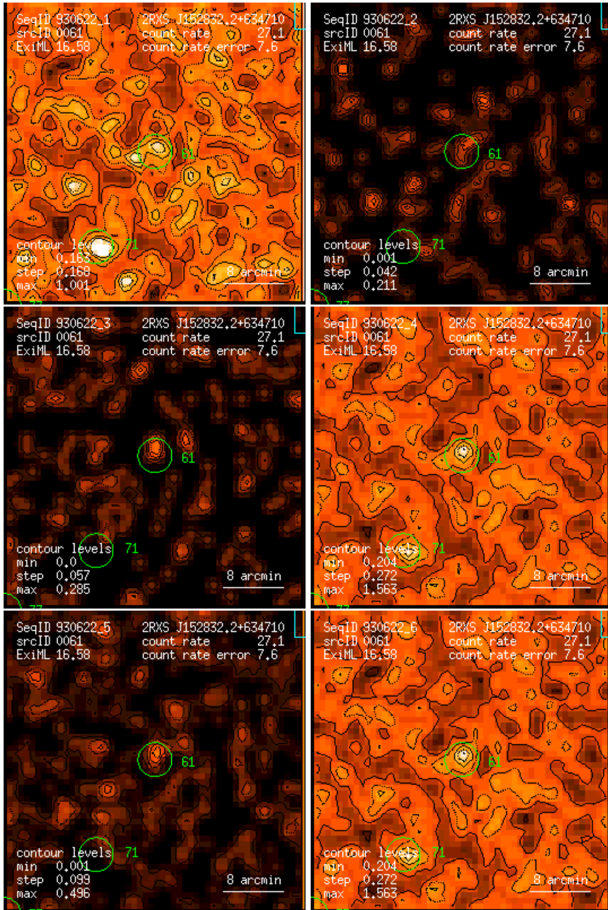
Figure 61: RASS 930622: detection 0061: band rate images, Gaussian filter: (1) PSPC channels 11 – 41, (2) 52 – 90, (3) 91 – 201, (4) 11 – 235, (5) 52 – 201, (6) 11 – 201. Broad band rates in counts/ks. Band rate contour levels in counts/ks/arcmin 2 .
