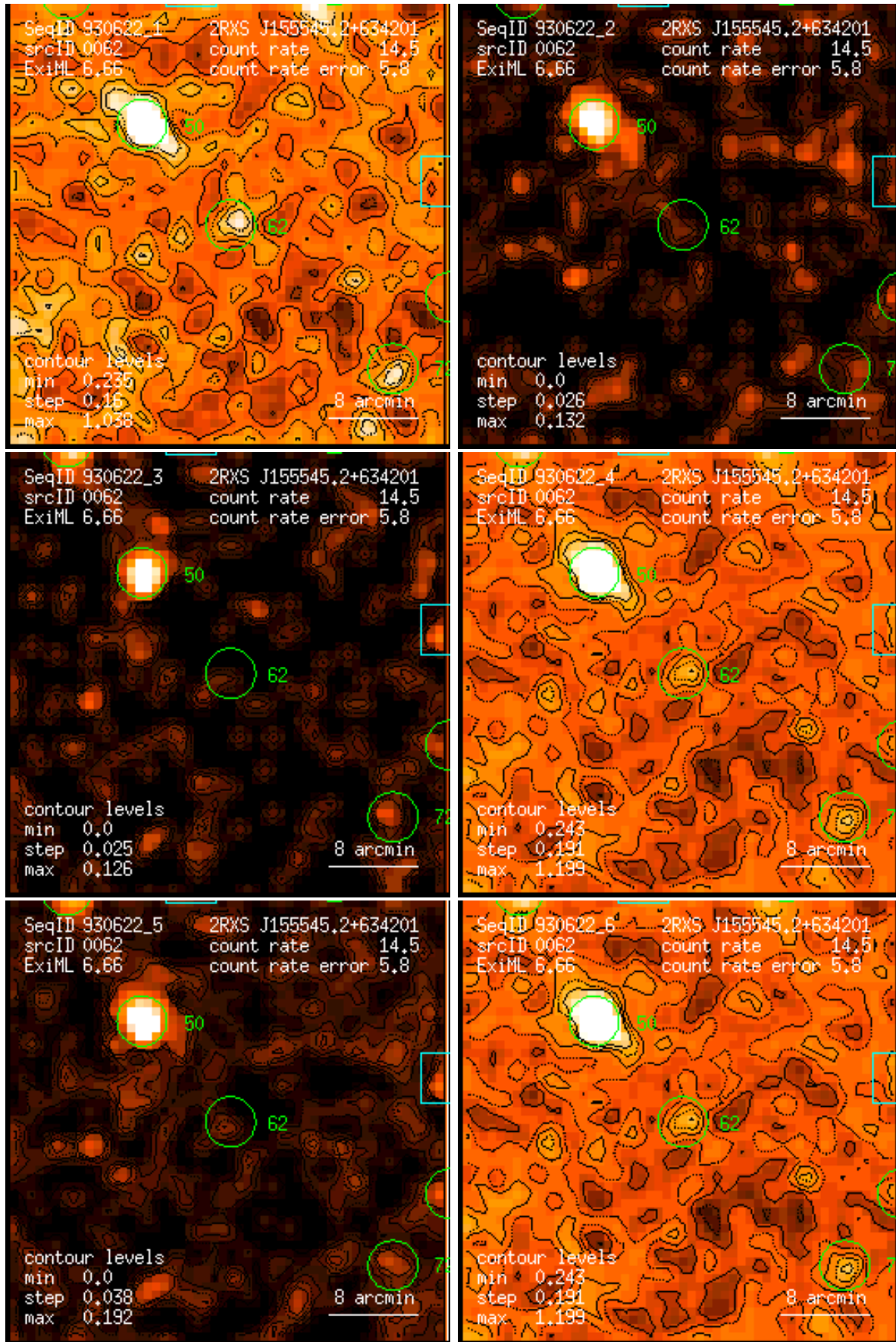
Figure 62: RASS 930622: detection 0062: band rate images, Gaussian filter: (1) PSPC channels 11 – 41, (2) 52 – 90, (3) 91 – 201, (4) 11 – 235, (5) 52 – 201, (6) 11 – 201. Broad band rates in counts/ks. Band rate contour levels in counts/ks/arcmin 2 .
