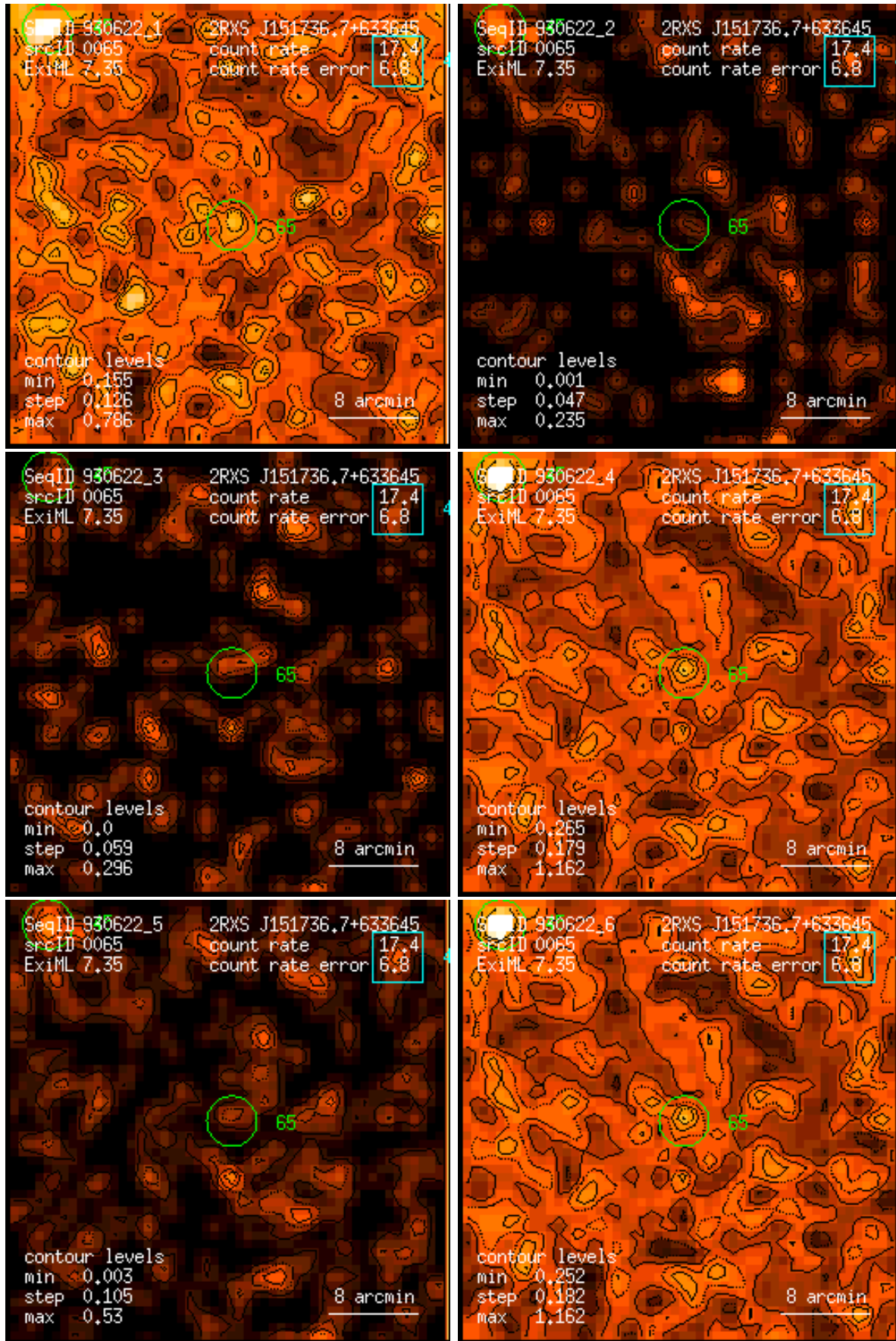
Figure 65: RASS 930622: detection 0065: band rate images, Gaussian filter: (1) PSPC channels 11 – 41, (2) 52 – 90, (3) 91 – 201, (4) 11 – 235, (5) 52 – 201, (6) 11 – 201. Broad band rates in counts/ks. Band rate contour levels in counts/ks/arcmin 2 .
