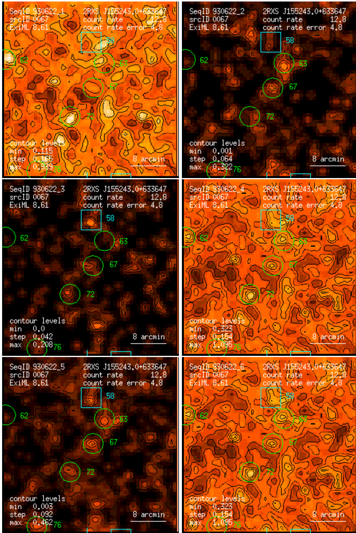
Figure 67: RASS 930622: detection 0067: band rate images, Gaussian filter: (1) PSPC channels 11 – 41, (2) 52 – 90, (3) 91 – 201, (4) 11 – 235, (5) 52 – 201, (6) 11 – 201. Broad band rates in counts/ks. Band rate contour levels in counts/ks/arcmin 2 .
