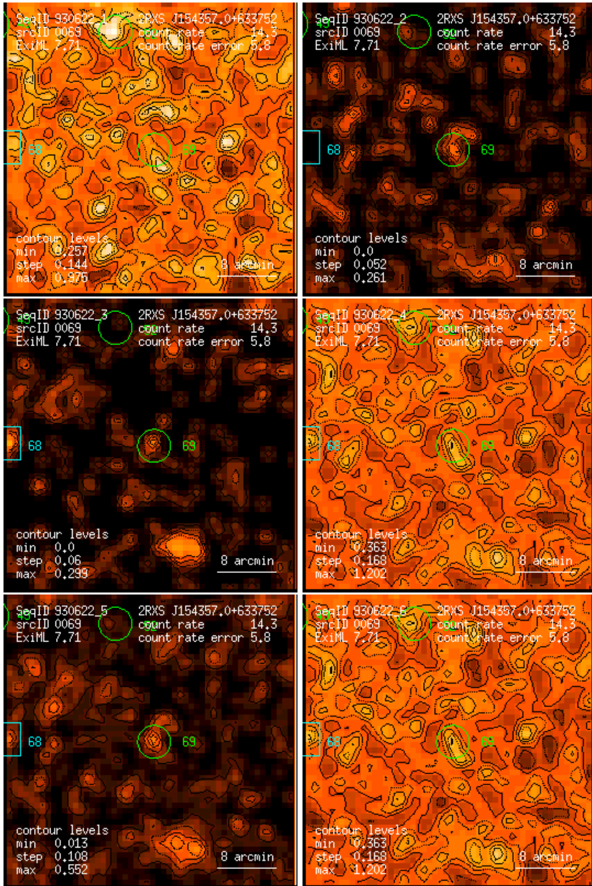
Figure 69: RASS 930622: detection 0069: band rate images, Gaussian filter: (1) PSPC channels 11 – 41, (2) 52 – 90, (3) 91 – 201, (4) 11 – 235, (5) 52 – 201, (6) 11 – 201. Broad band rates in counts/ks. Band rate contour levels in counts/ks/arcmin 2 .
