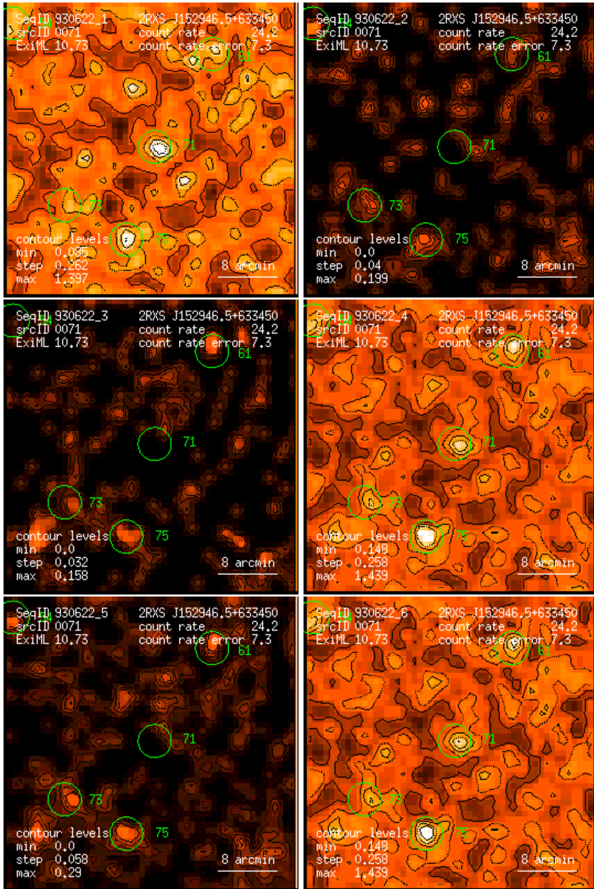
Figure 71: RASS 930622: detection 0071: band rate images, Gaussian filter: (1) PSPC channels 11 – 41, (2) 52 – 90, (3) 91 – 201, (4) 11 – 235, (5) 52 – 201, (6) 11 – 201. Broad band rates in counts/ks. Band rate contour levels in counts/ks/arcmin 2 .
