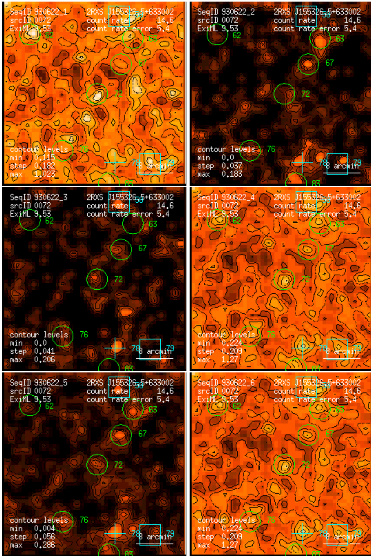
Figure 72: RASS 930622: detection 0072: band rate images, Gaussian filter: (1) PSPC channels 11 – 41, (2) 52 – 90, (3) 91 – 201, (4) 11 – 235, (5) 52 – 201, (6) 11 – 201. Broad band rates in counts/ks. Band rate contour levels in counts/ks/arcmin 2 .
