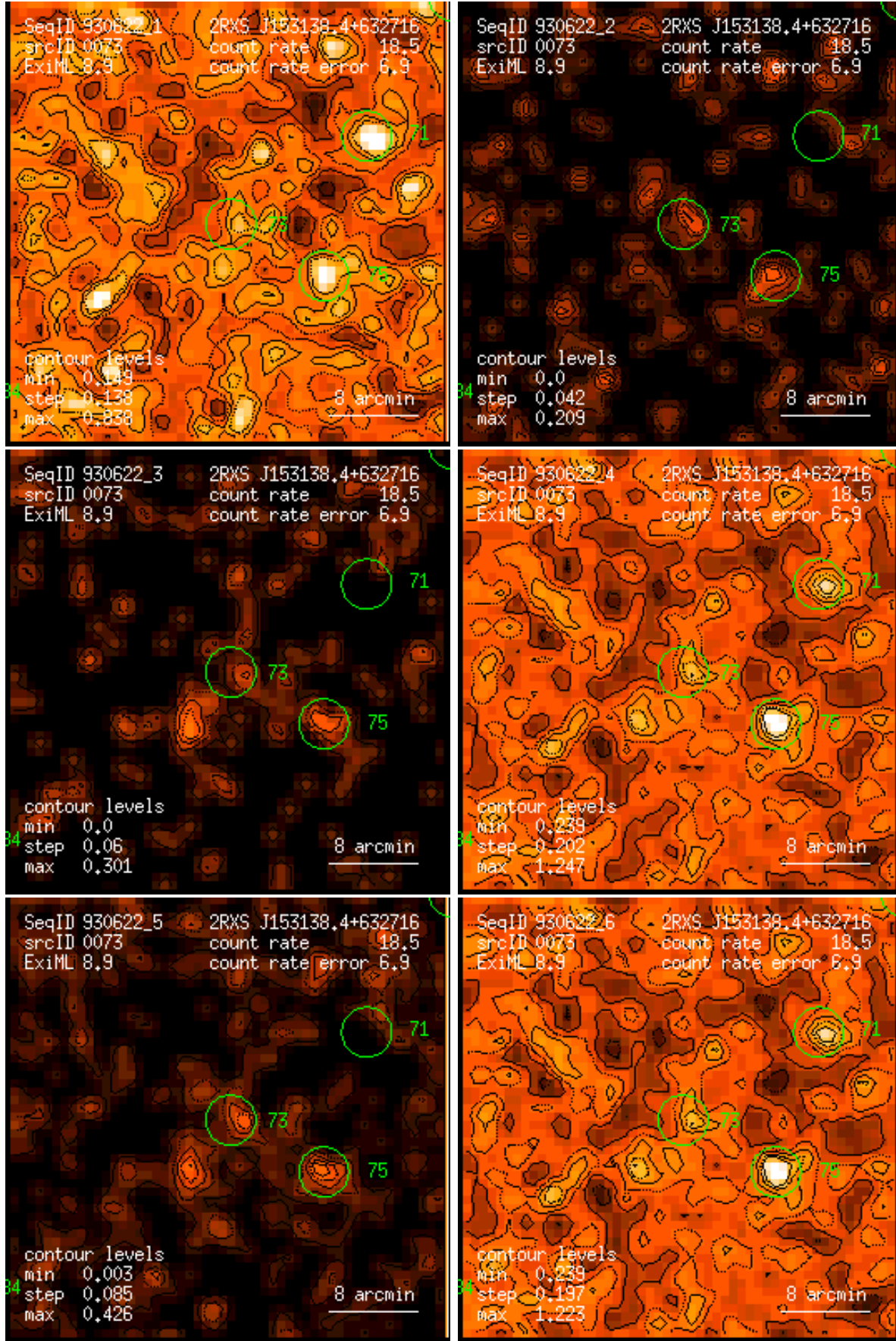
Figure 73: RASS 930622: detection 0073: band rate images, Gaussian filter: (1) PSPC channels 11 – 41, (2) 52 – 90, (3) 91 – 201, (4) 11 – 235, (5) 52 – 201, (6) 11 – 201. Broad band rates in counts/ks. Band rate contour levels in counts/ks/arcmin 2 .
