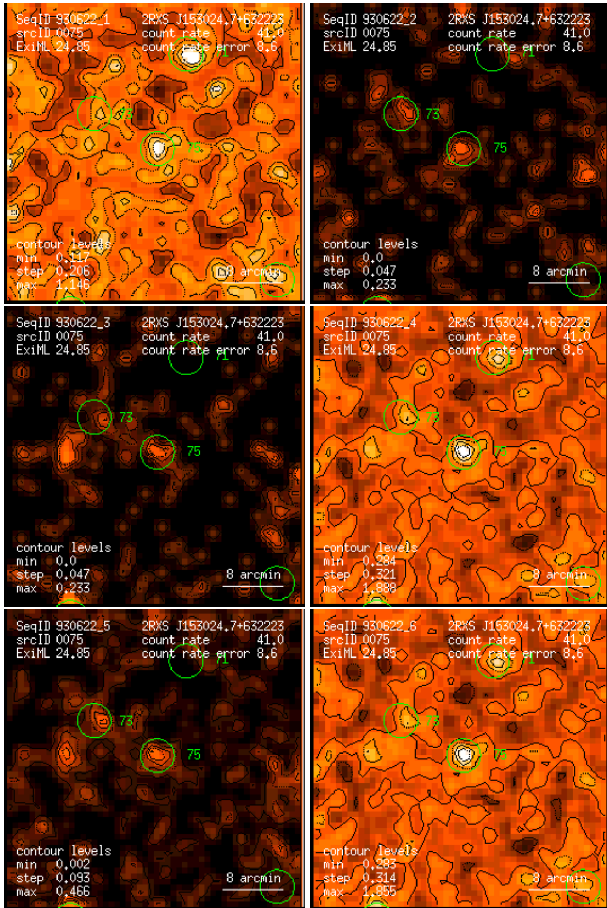
Figure 75: RASS 930622: detection 0075: band rate images, Gaussian filter: (1) PSPC channels 11 – 41, (2) 52 – 90, (3) 91 – 201, (4) 11 – 235, (5) 52 – 201, (6) 11 – 201. Broad band rates in counts/ks. Band rate contour levels in counts/ks/arcmin 2 .
