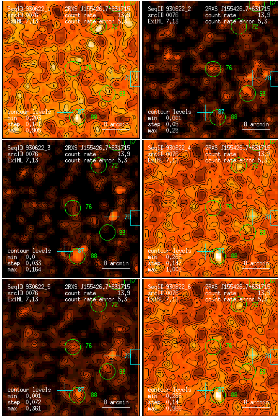
Figure 76: RASS 930622: detection 0076: band rate images, Gaussian filter: (1) PSPC channels 11 – 41, (2) 52 – 90, (3) 91 – 201, (4) 11 – 235, (5) 52 – 201, (6) 11 – 201. Broad band rates in counts/ks. Band rate contour levels in counts/ks/arcmin 2 .
