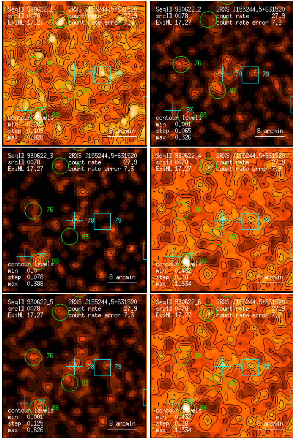
Figure 78: RASS 930622: detection 0078: band rate images, Gaussian filter: (1) PSPC channels 11 – 41, (2) 52 – 90, (3) 91 – 201, (4) 11 – 235, (5) 52 – 201, (6) 11 – 201. Broad band rates in counts/ks. Band rate contour levels in counts/ks/arcmin 2 .
