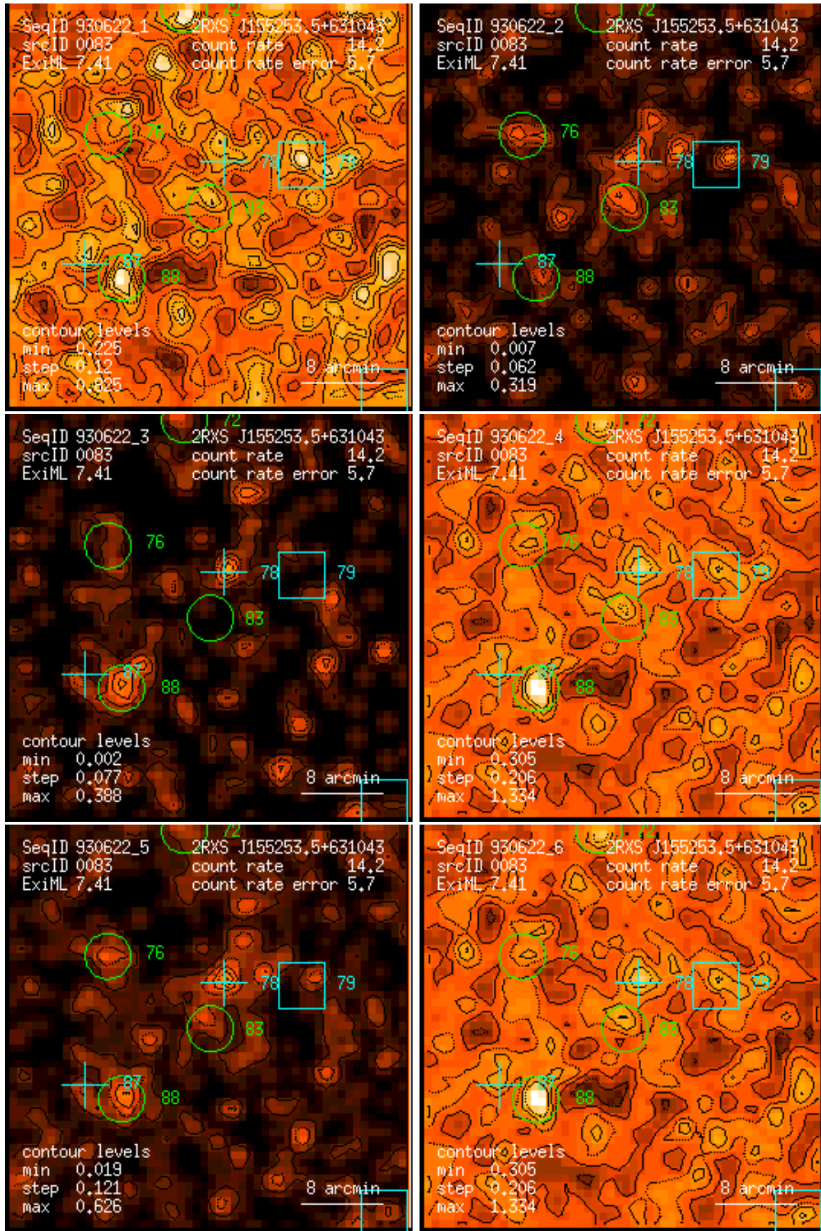
Figure 83: RASS 930622: detection 0083: band rate images, Gaussian filter: (1) PSPC channels 11 – 41, (2) 52 – 90, (3) 91 – 201, (4) 11 – 235, (5) 52 – 201, (6) 11 – 201. Broad band rates in counts/ks. Band rate contour levels in counts/ks/arcmin 2 .
