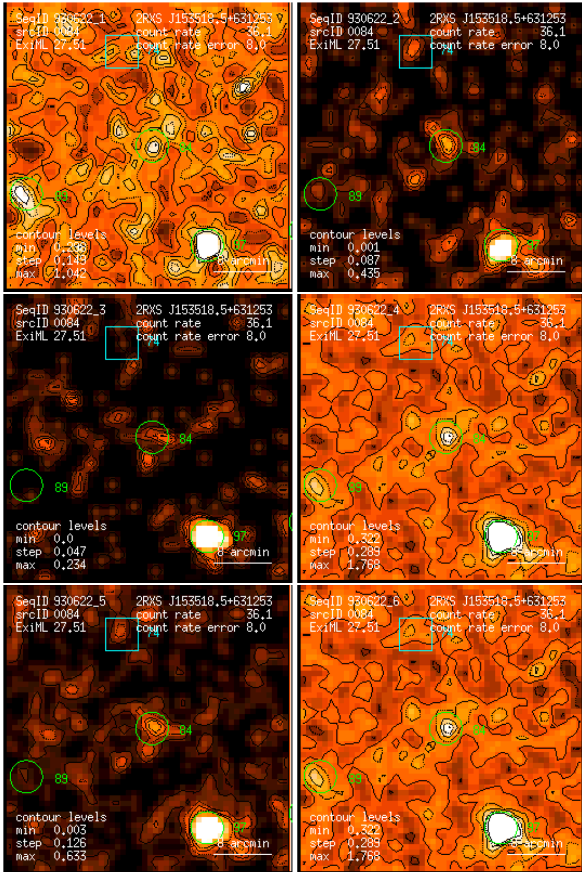
Figure 84: RASS 930622: detection 0084: band rate images, Gaussian filter: (1) PSPC channels 11 – 41, (2) 52 – 90, (3) 91 – 201, (4) 11 – 235, (5) 52 – 201, (6) 11 – 201. Broad band rates in counts/ks. Band rate contour levels in counts/ks/arcmin 2 .
