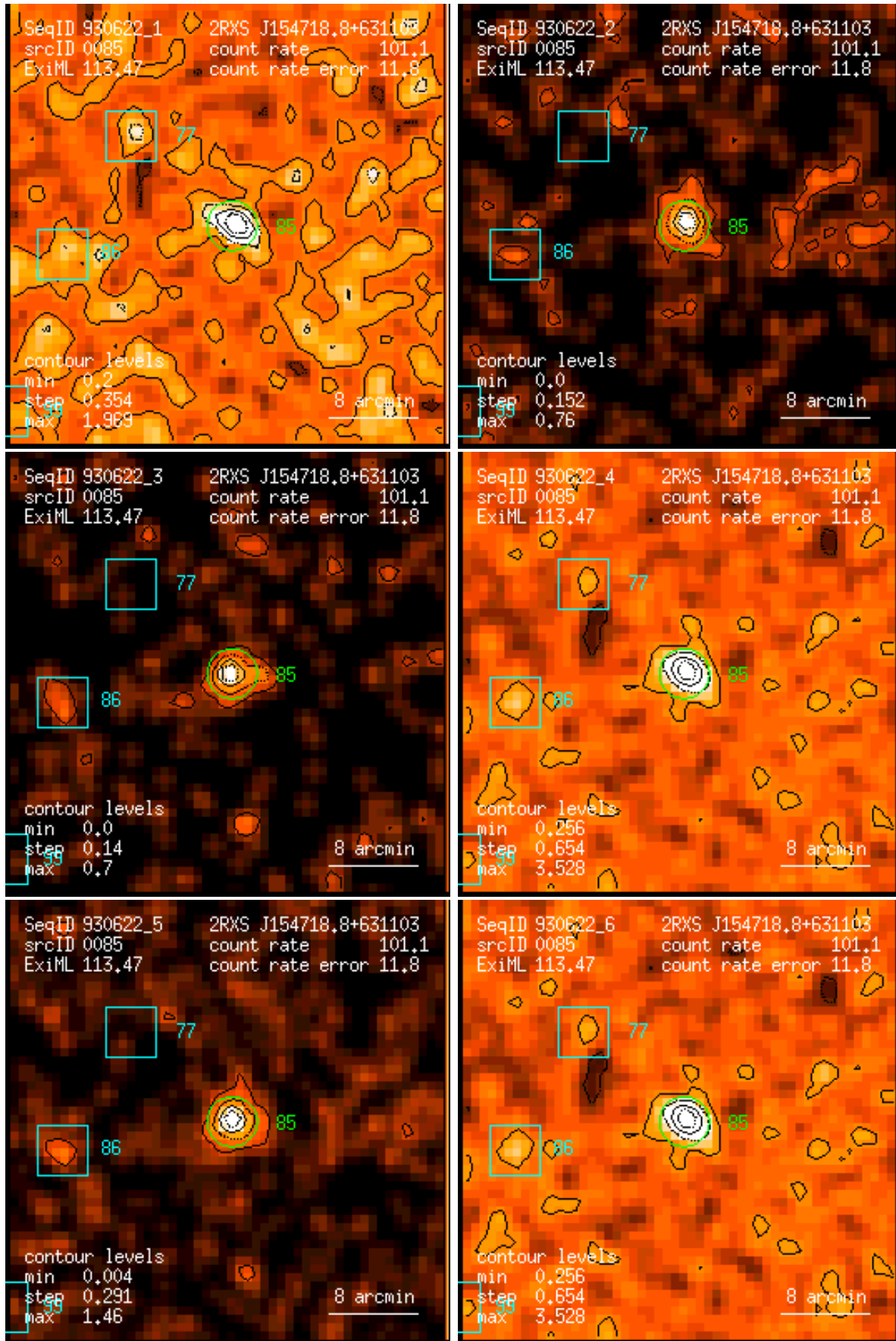
Figure 85: RASS 930622: detection 0085: band rate images, Gaussian filter: (1) PSPC channels 11 – 41, (2) 52 – 90, (3) 91 – 201, (4) 11 – 235, (5) 52 – 201, (6) 11 – 201. Broad band rates in counts/ks. Band rate contour levels in counts/ks/arcmin 2 .
