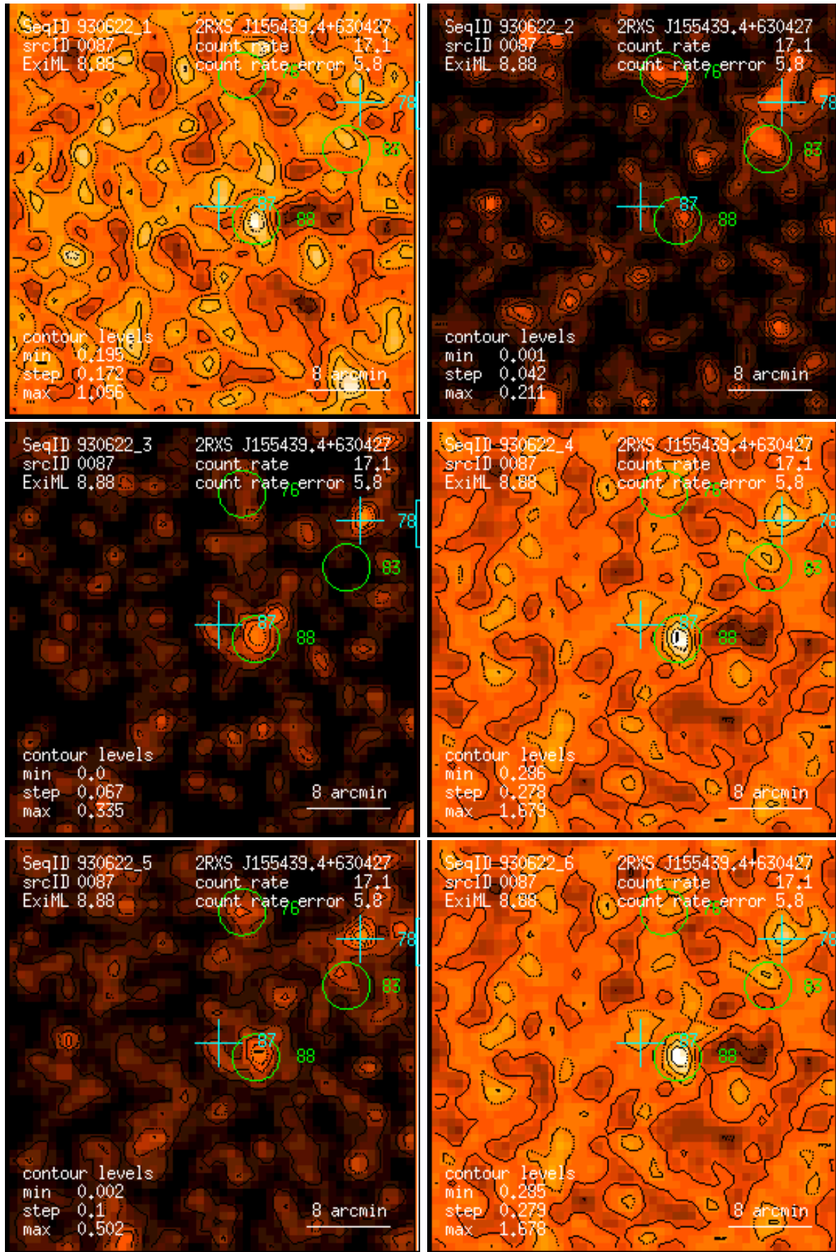
Figure 87: RASS 930622: detection 0087: band rate images, Gaussian filter: (1) PSPC channels 11 – 41, (2) 52 – 90, (3) 91 – 201, (4) 11 – 235, (5) 52 – 201, (6) 11 – 201. Broad band rates in counts/ks. Band rate contour levels in counts/ks/arcmin 2 .
