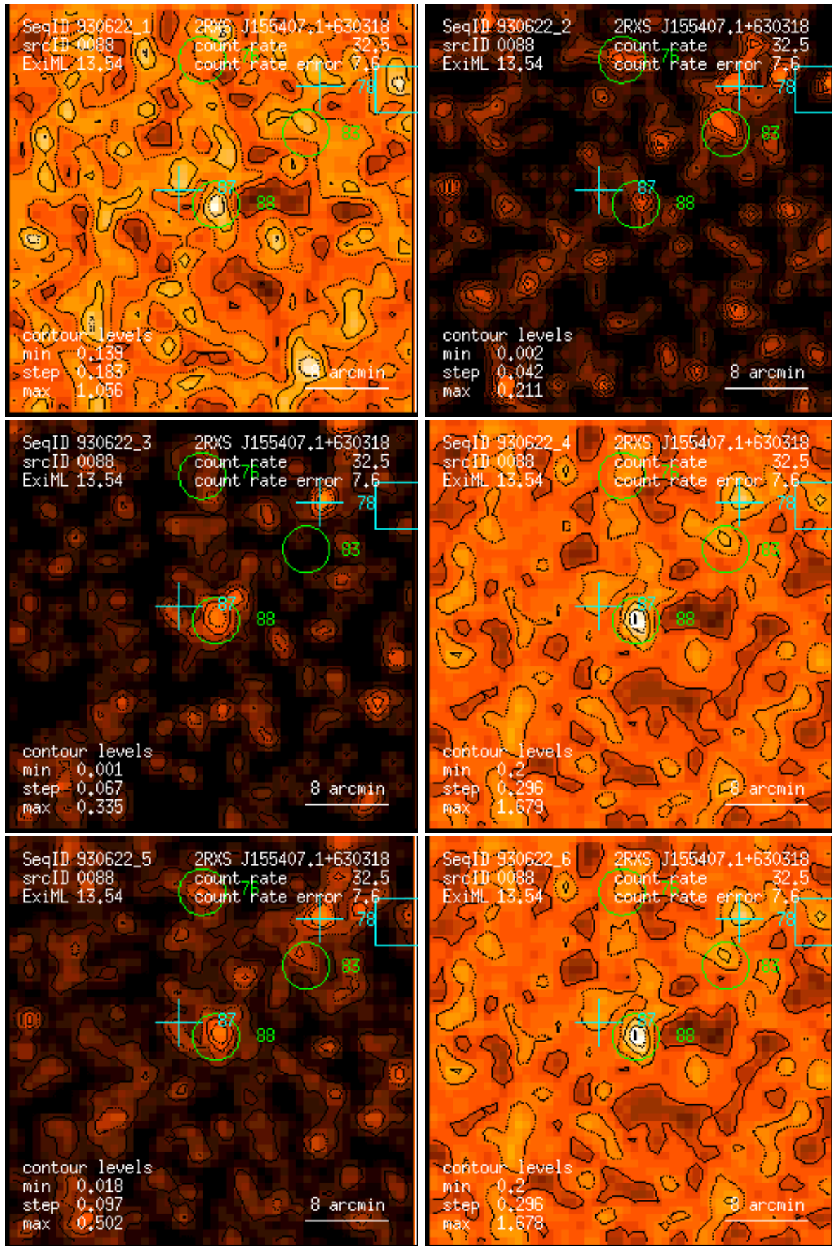
Figure 88: RASS 930622: detection 0088: band rate images, Gaussian filter: (1) PSPC channels 11 – 41, (2) 52 – 90, (3) 91 – 201, (4) 11 – 235, (5) 52 – 201, (6) 11 – 201. Broad band rates in counts/ks. Band rate contour levels in counts/ks/arcmin 2 .
