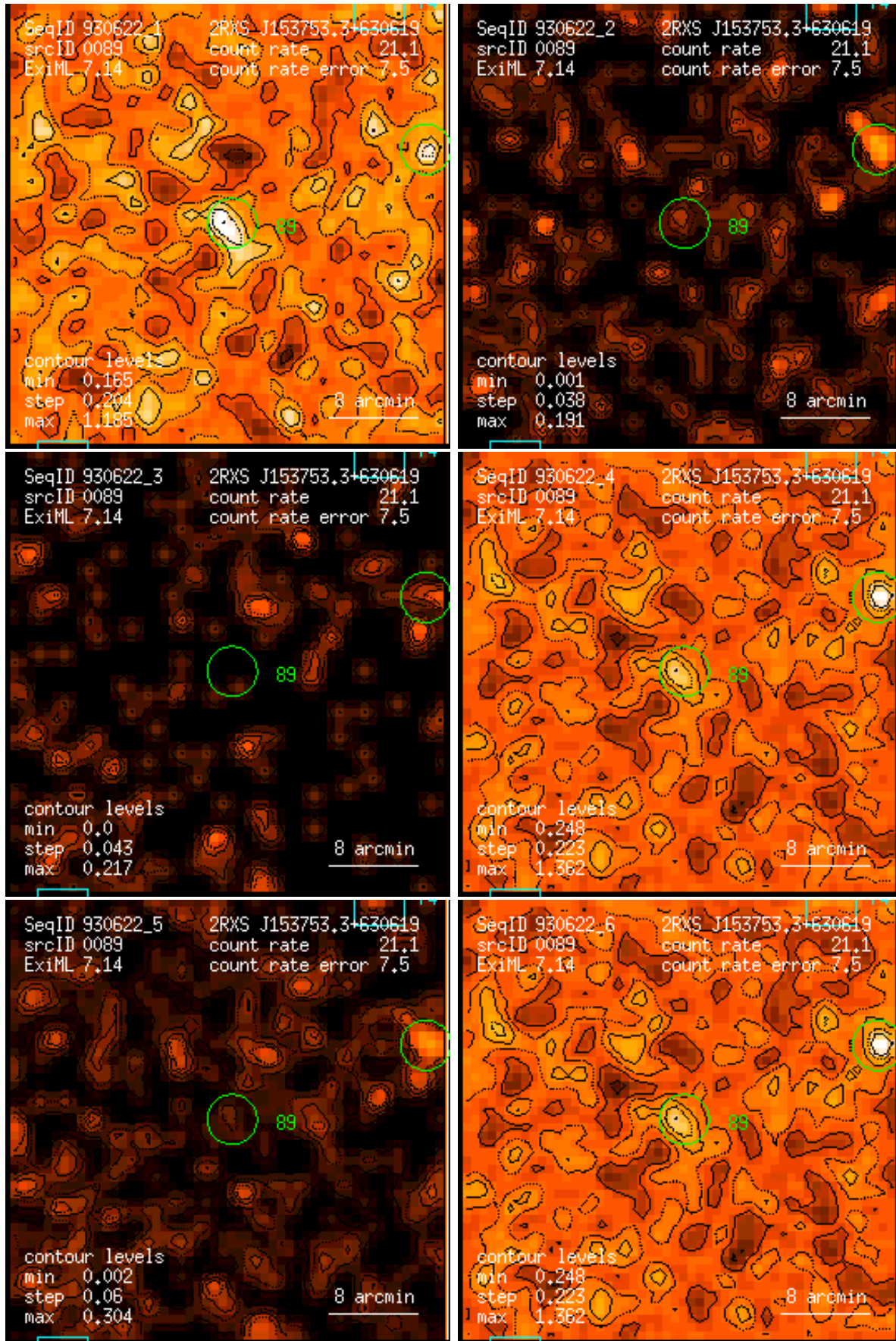
Figure 89: RASS 930622: detection 0089: band rate images, Gaussian filter: (1) PSPC channels 11 – 41, (2) 52 – 90, (3) 91 – 201, (4) 11 – 235, (5) 52 – 201, (6) 11 – 201. Broad band rates in counts/ks. Band rate contour levels in counts/ks/arcmin 2 .
