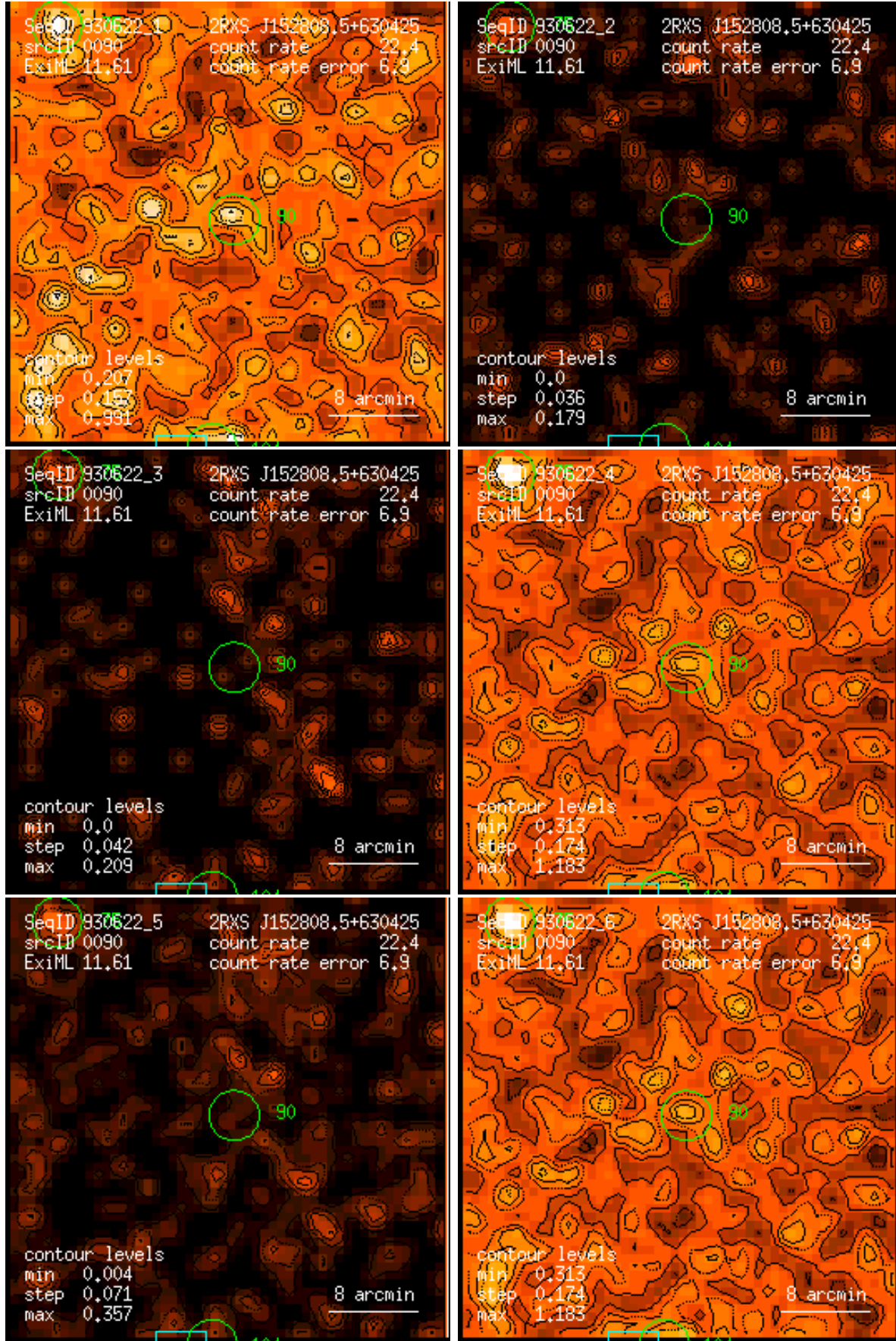
Figure 90: RASS 930622: detection 0090: band rate images, Gaussian filter: (1) PSPC channels 11 – 41, (2) 52 – 90, (3) 91 – 201, (4) 11 – 235, (5) 52 – 201, (6) 11 – 201. Broad band rates in counts/ks. Band rate contour levels in counts/ks/arcmin 2 .
