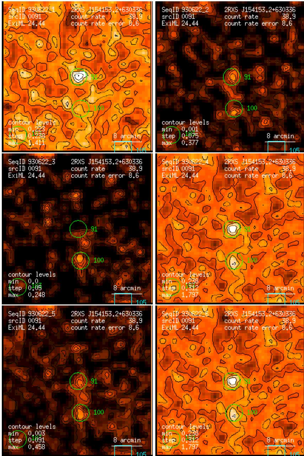
Figure 91: RASS 930622: detection 0091: band rate images, Gaussian filter: (1) PSPC channels 11 – 41, (2) 52 – 90, (3) 91 – 201, (4) 11 – 235, (5) 52 – 201, (6) 11 – 201. Broad band rates in counts/ks. Band rate contour levels in counts/ks/arcmin 2 .
