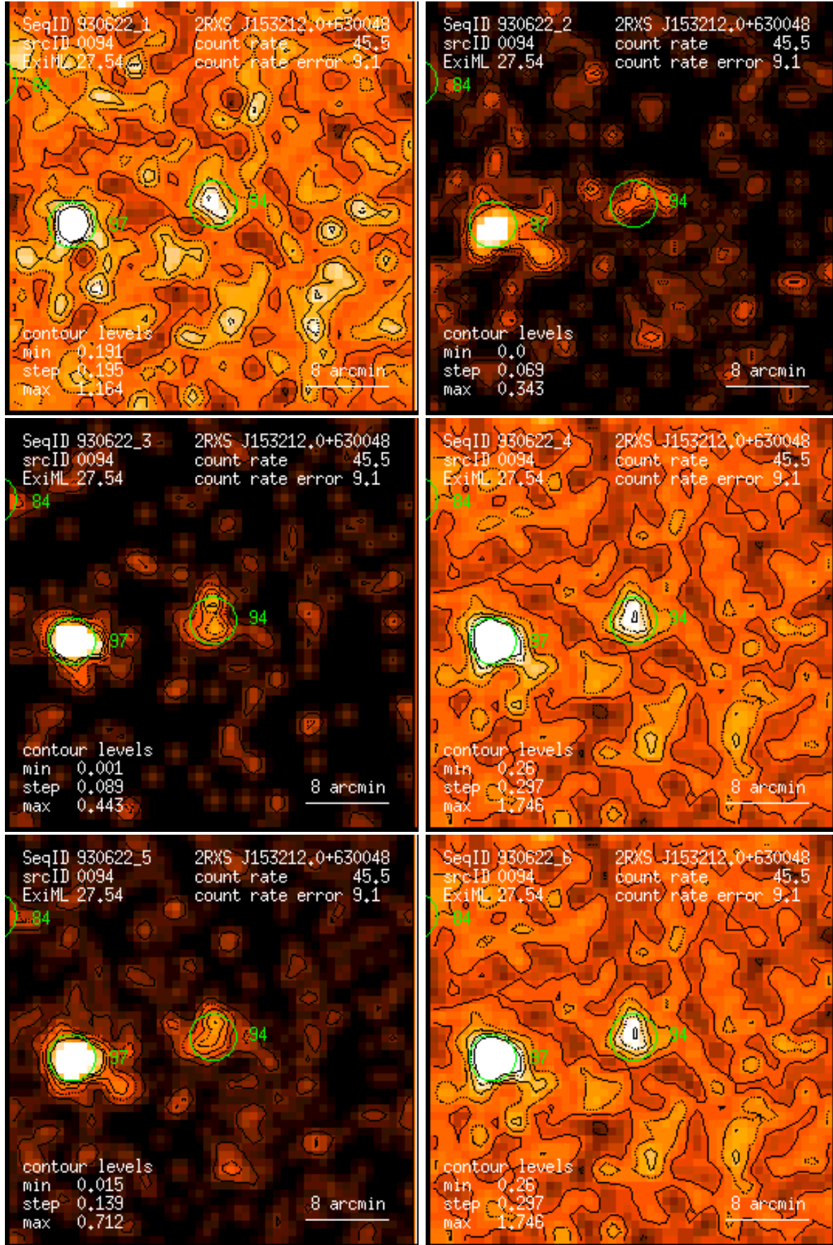
Figure 94: RASS 930622: detection 0094: band rate images, Gaussian filter: (1) PSPC channels 11 – 41, (2) 52 – 90, (3) 91 – 201, (4) 11 – 235, (5) 52 – 201, (6) 11 – 201. Broad band rates in counts/ks. Band rate contour levels in counts/ks/arcmin 2 .
