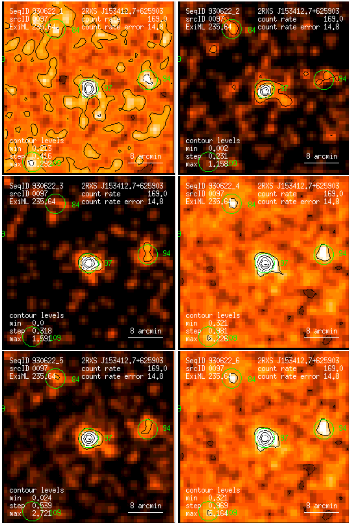
Figure 97: RASS 930622: detection 0097: band rate images, Gaussian filter: (1) PSPC channels 11 – 41, (2) 52 – 90, (3) 91 – 201, (4) 11 – 235, (5) 52 – 201, (6) 11 – 201. Broad band rates in counts/ks. Band rate contour levels in counts/ks/arcmin 2 .
