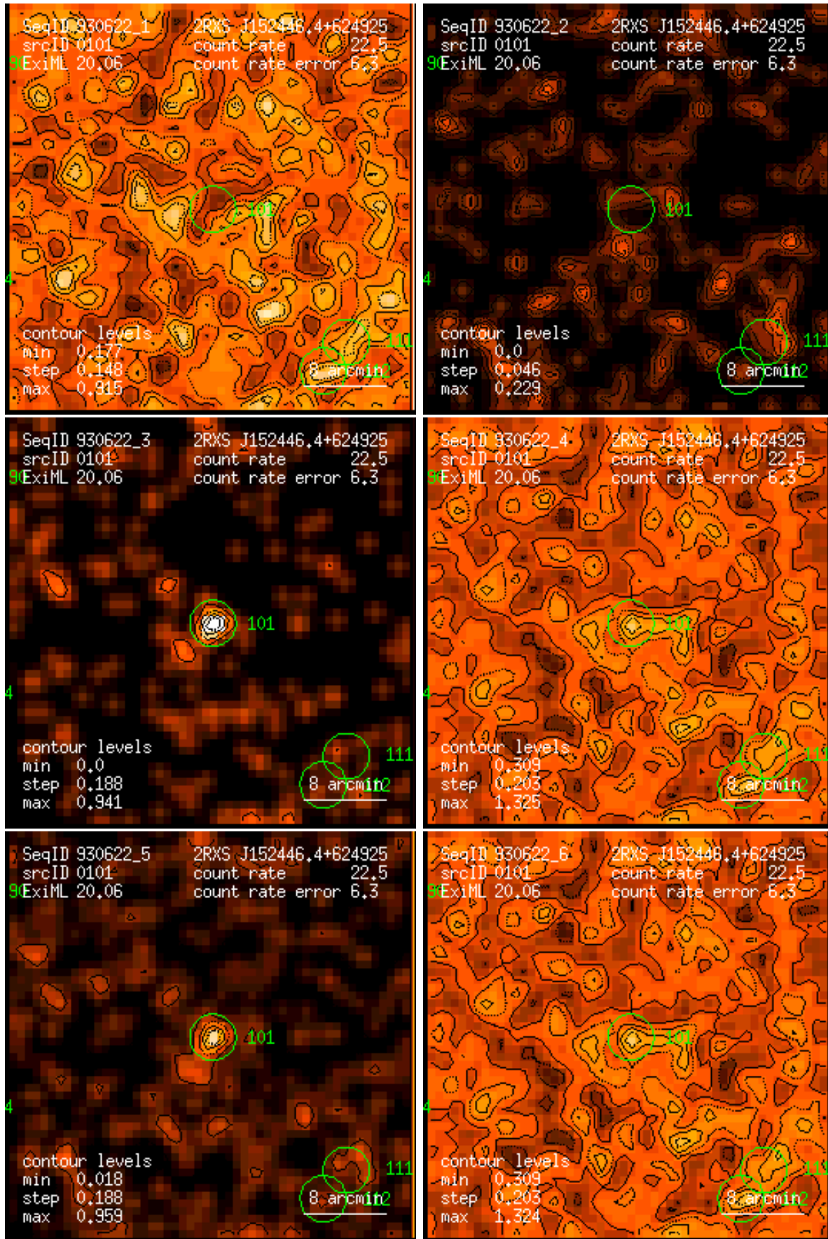
Figure 101: RASS 930622: detection 0101: band rate images, Gaussian filter: (1) PSPC channels 11 – 41, (2) 52 – 90, (3) 91 – 201, (4) 11 – 235, (5) 52 – 201, (6) 11 – 201. Broad band rates in counts/ks. Band rate contour levels in counts/ks/arcmin 2 .
