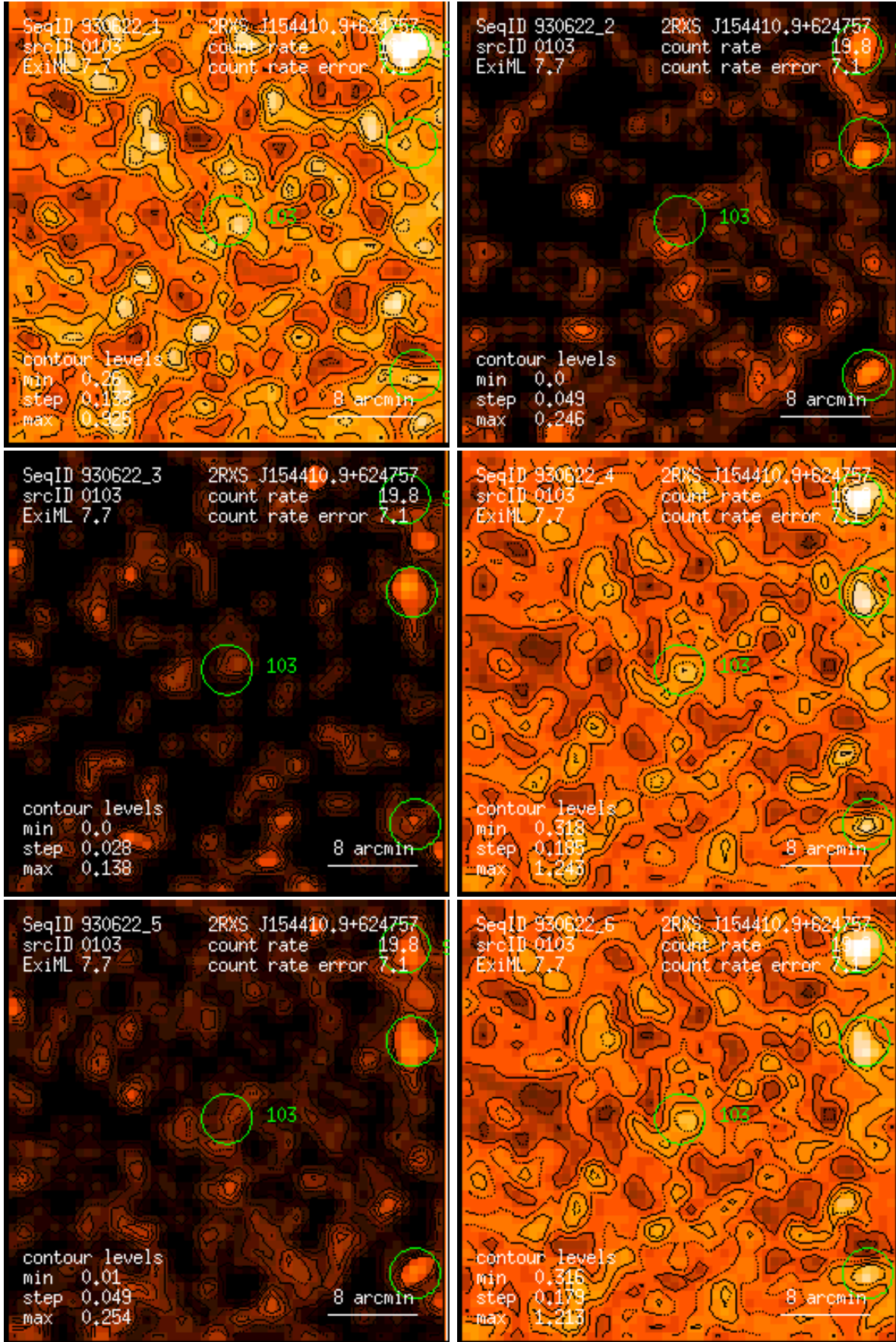
Figure 103: RASS 930622: detection 0103: band rate images, Gaussian filter: (1) PSPC channels 11 – 41, (2) 52 – 90, (3) 91 – 201, (4) 11 – 235, (5) 52 – 201, (6) 11 – 201. Broad band rates in counts/ks. Band rate contour levels in counts/ks/arcmin 2 .
