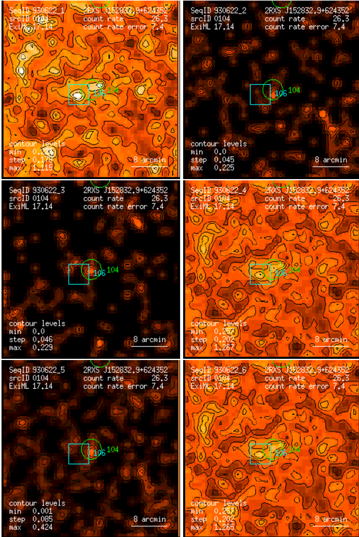
Figure 104: RASS 930622: detection 0104: band rate images, Gaussian filter: (1) PSPC channels 11 – 41, (2) 52 – 90, (3) 91 – 201, (4) 11 – 235, (5) 52 – 201, (6) 11 – 201. Broad band rates in counts/ks. Band rate contour levels in counts/ks/arcmin 2 .
