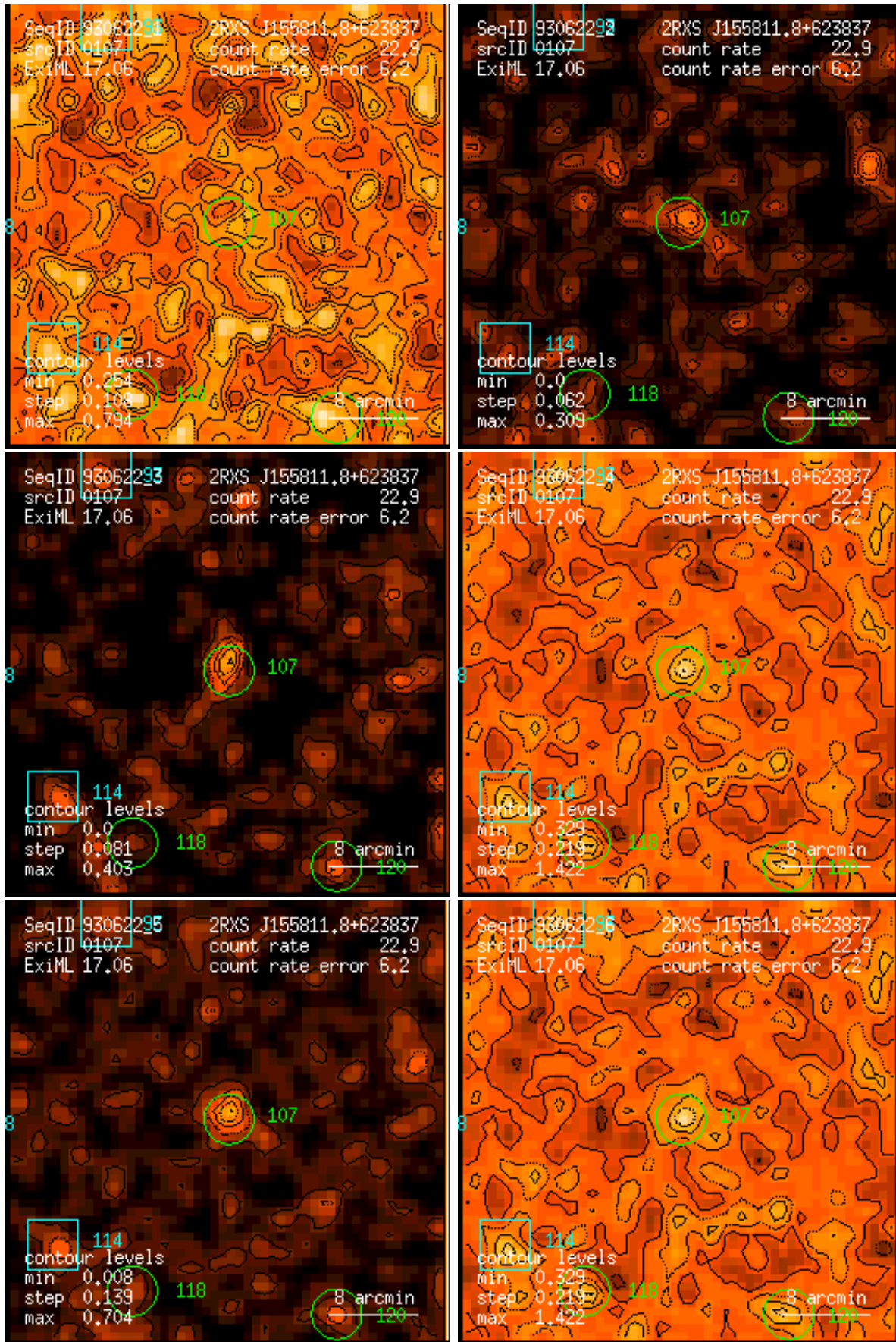
Figure 107: RASS 930622: detection 0107: band rate images, Gaussian filter: (1) PSPC channels 11 – 41, (2) 52 – 90, (3) 91 – 201, (4) 11 – 235, (5) 52 – 201, (6) 11 – 201. Broad band rates in counts/ks. Band rate contour levels in counts/ks/arcmin 2 .
