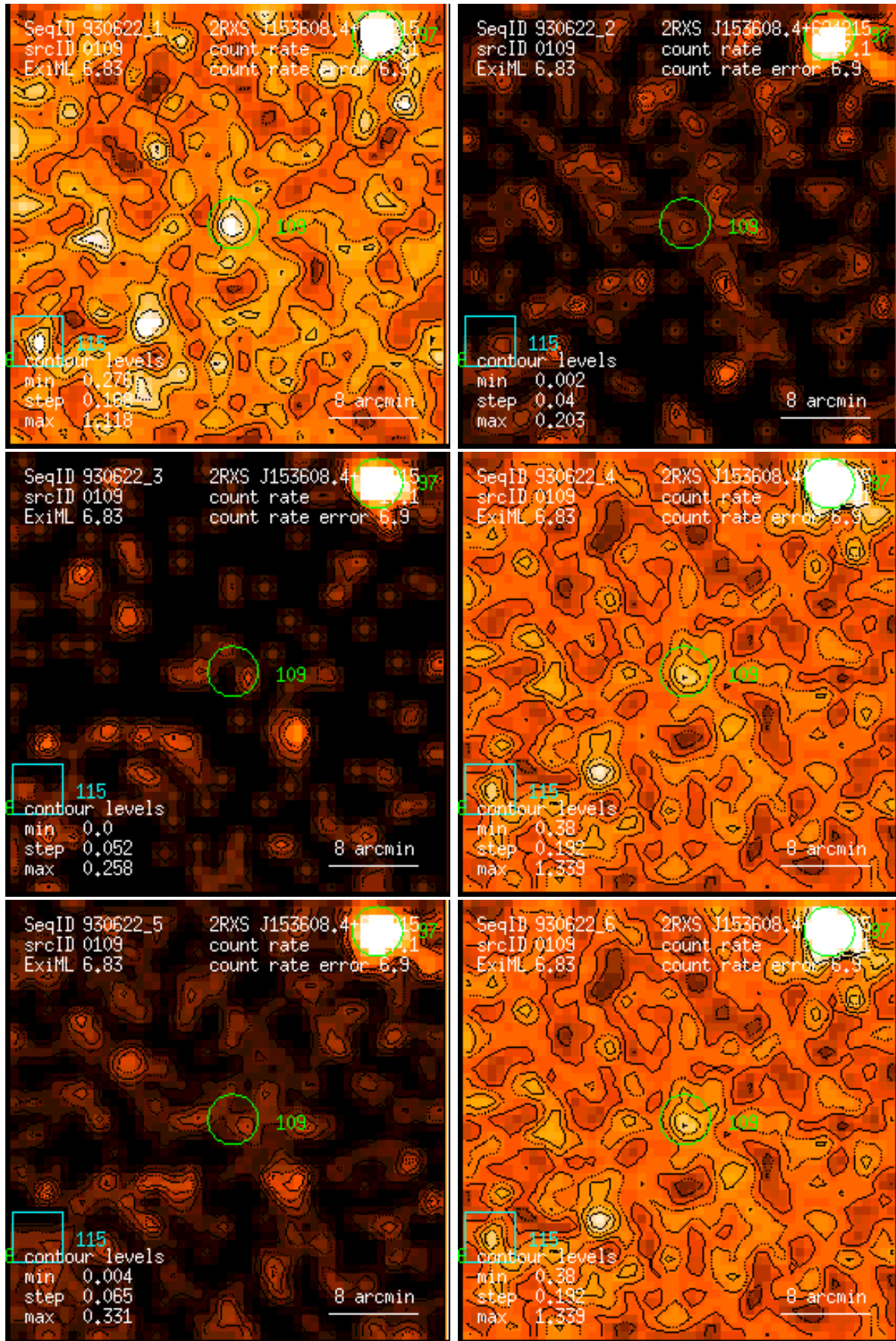
Figure 109: RASS 930622: detection 0109: band rate images, Gaussian filter: (1) PSPC channels 11 – 41, (2) 52 – 90, (3) 91 – 201, (4) 11 – 235, (5) 52 – 201, (6) 11 – 201. Broad band rates in counts/ks. Band rate contour levels in counts/ks/arcmin 2 .
