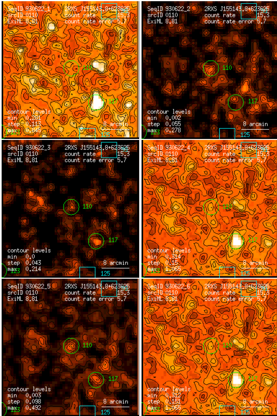
Figure 110: RASS 930622: detection 0110: band rate images, Gaussian filter: (1) PSPC channels 11 – 41, (2) 52 – 90, (3) 91 – 201, (4) 11 – 235, (5) 52 – 201, (6) 11 – 201. Broad band rates in counts/ks. Band rate contour levels in counts/ks/arcmin 2 .
