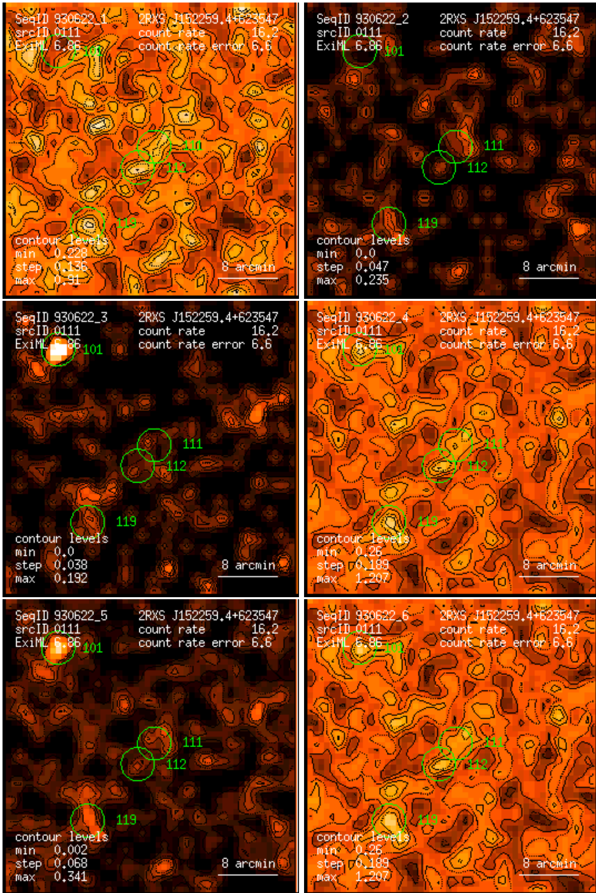
Figure 111: RASS 930622: detection 0111: band rate images, Gaussian filter: (1) PSPC channels 11 – 41, (2) 52 – 90, (3) 91 – 201, (4) 11 – 235, (5) 52 – 201, (6) 11 – 201. Broad band rates in counts/ks. Band rate contour levels in counts/ks/arcmin 2 .
