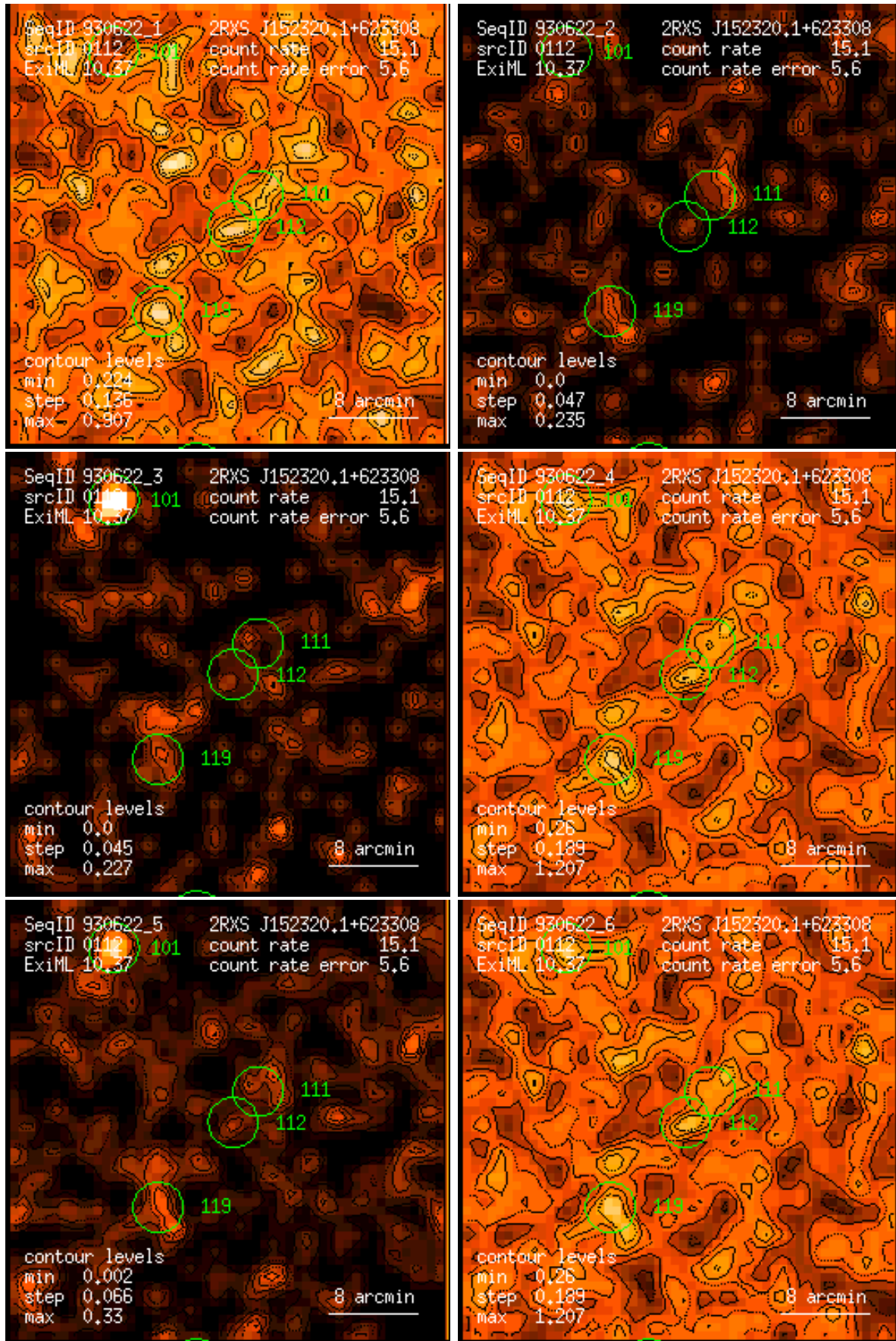
Figure 112: RASS 930622: detection 0112: band rate images, Gaussian filter: (1) PSPC channels 11 – 41, (2) 52 – 90, (3) 91 – 201, (4) 11 – 235, (5) 52 – 201, (6) 11 – 201. Broad band rates in counts/ks. Band rate contour levels in counts/ks/arcmin 2 .
