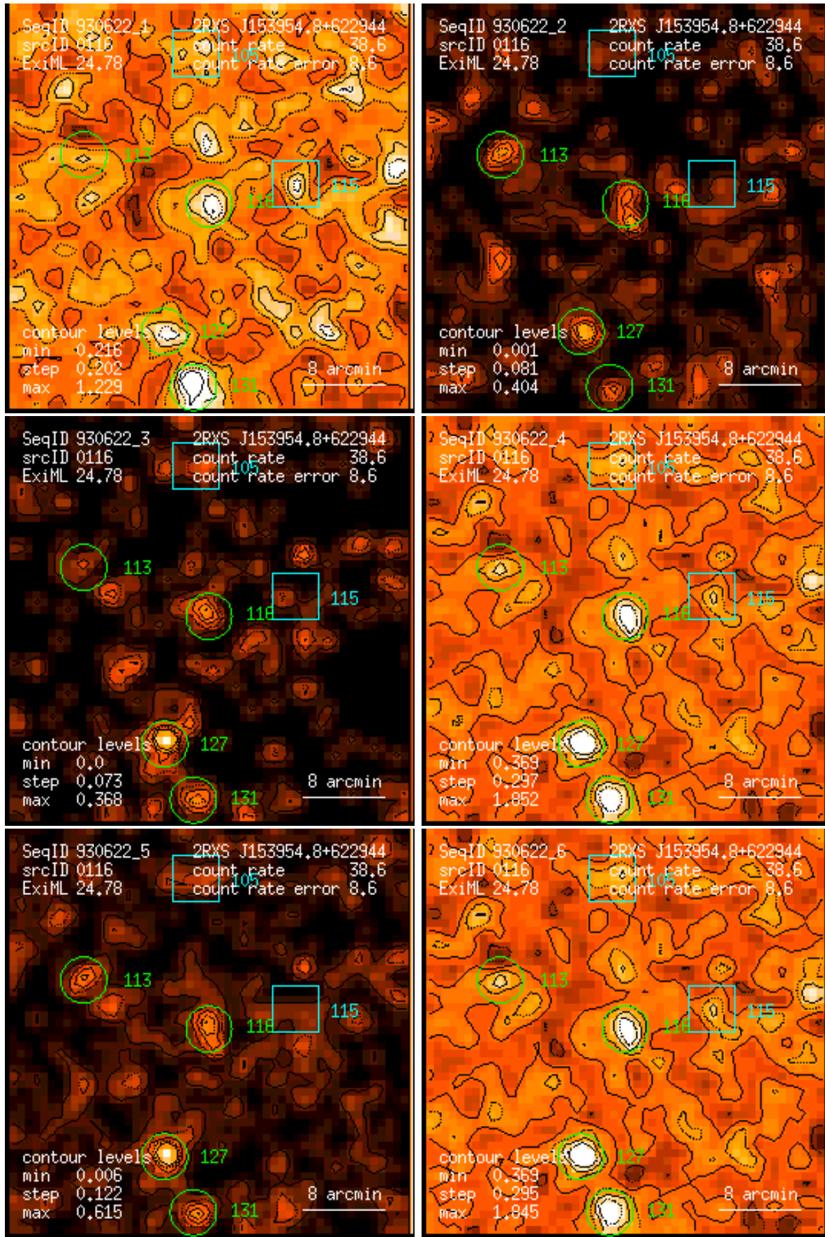
Figure 116: RASS 930622: detection 0116: band rate images, Gaussian filter: (1) PSPC channels 11 – 41, (2) 52 – 90, (3) 91 – 201, (4) 11 – 235, (5) 52 – 201, (6) 11 – 201. Broad band rates in counts/ks. Band rate contour levels in counts/ks/arcmin 2 .
