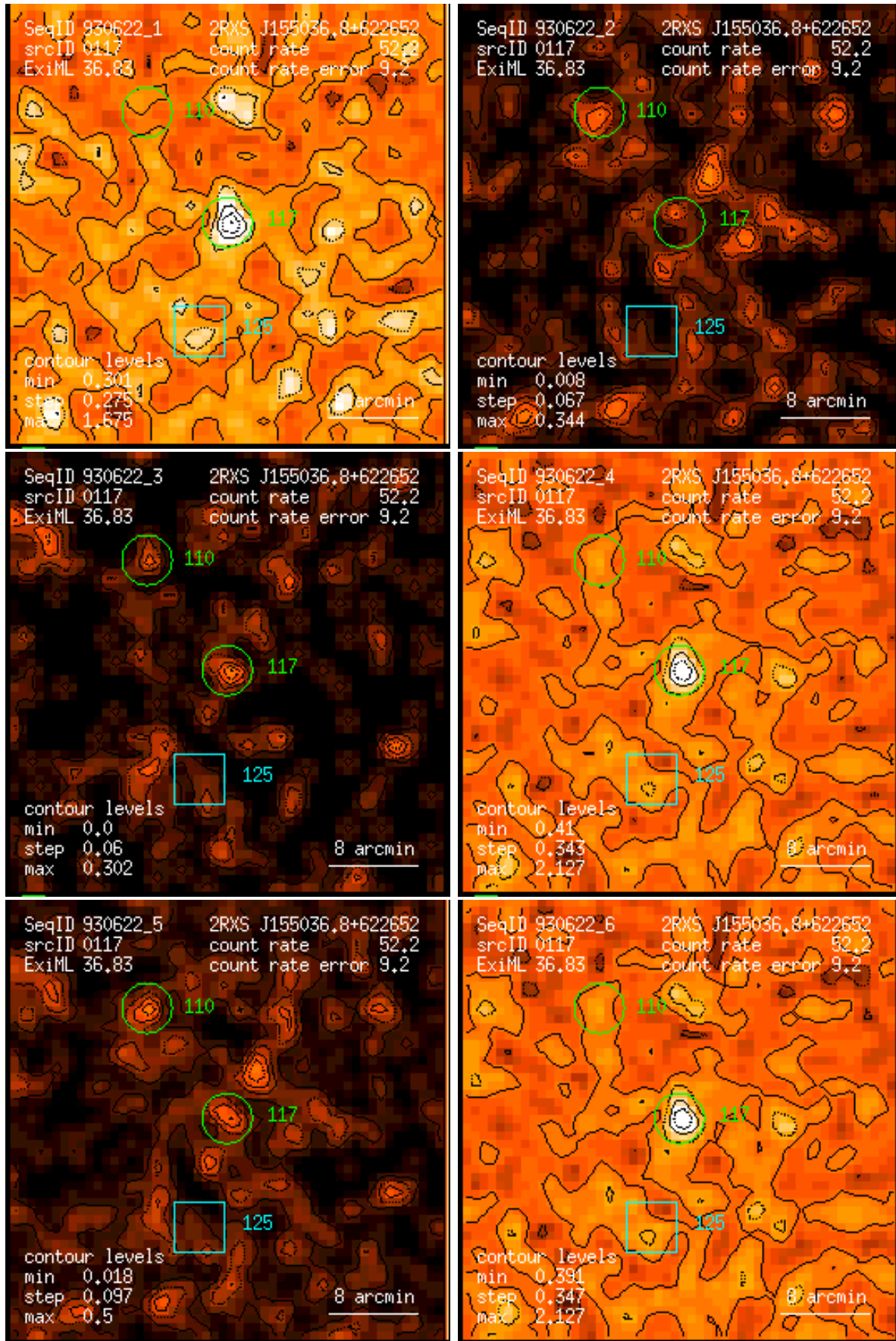
Figure 117: RASS 930622: detection 0117: band rate images, Gaussian filter: (1) PSPC channels 11 – 41, (2) 52 – 90, (3) 91 – 201, (4) 11 – 235, (5) 52 – 201, (6) 11 – 201. Broad band rates in counts/ks. Band rate contour levels in counts/ks/arcmin 2 .
