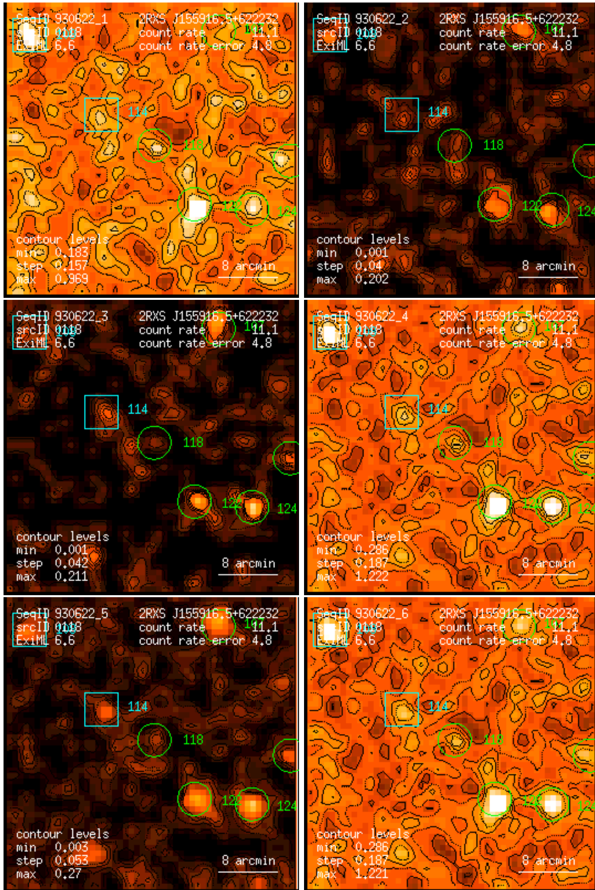
Figure 118: RASS 930622: detection 0118: band rate images, Gaussian filter: (1) PSPC channels 11 – 41, (2) 52 – 90, (3) 91 – 201, (4) 11 – 235, (5) 52 – 201, (6) 11 – 201. Broad band rates in counts/ks. Band rate contour levels in counts/ks/arcmin 2 .
