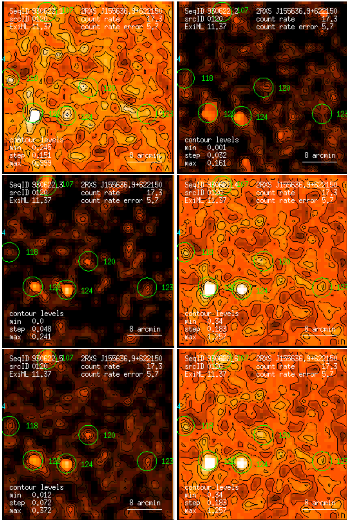
Figure 120: RASS 930622: detection 0120: band rate images, Gaussian filter: (1) PSPC channels 11 – 41, (2) 52 – 90, (3) 91 – 201, (4) 11 – 235, (5) 52 – 201, (6) 11 – 201. Broad band rates in counts/ks. Band rate contour levels in counts/ks/arcmin 2 .
